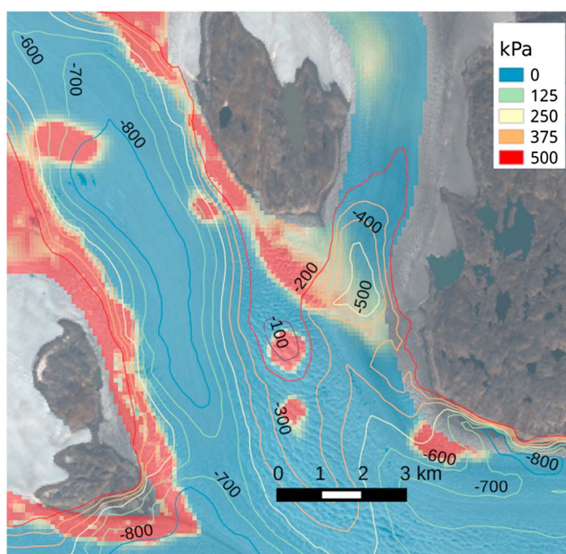
Figure 8. Bed elevation contours and stress of Helheim Glacier. The -100 m elevation contour coincides with a sticky spot.
