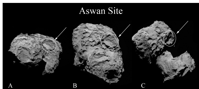
Fig. 1. OSIRIS NAC images taken on 6 August 2014 and showing the location of the Aswan site on the larger lobe of 67P. The first image of this set, A, was taken at 00.20.10 UT at a distance of 121.4 km and a scale of 2.3 m/px. Image B was taken at 02.20.12 UT, at a distance of 117.2 km and has a scale of 2.2 m/px, while the last one, C, was taken at 04.20.10 UT at a distance of 113.4 km and a scale of 2.1 m/px.
