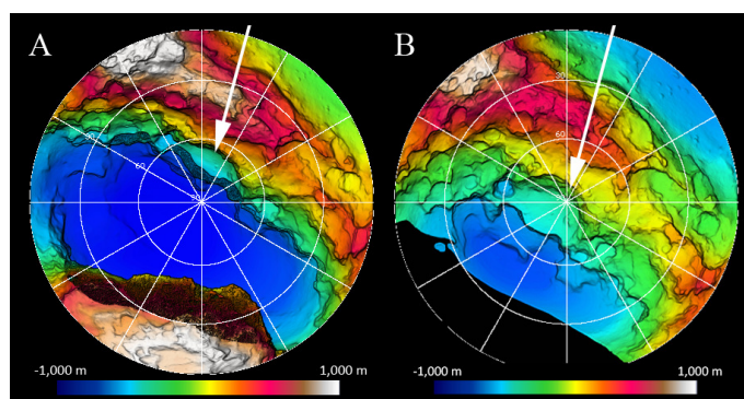
Fig. 2. A) Stereographic projection for the global 67P shape centered on the north pole. B) Stereographic projection for the large lobe of 67P (as identified in Preusker et al. 2015) centered on the corresponding north pole. The color coding shows the height above the 1500 m reference sphere: blue = -1000 m to red/white = 1000 m. The location of the Aswan site in both projections is indicated with white arrows.
