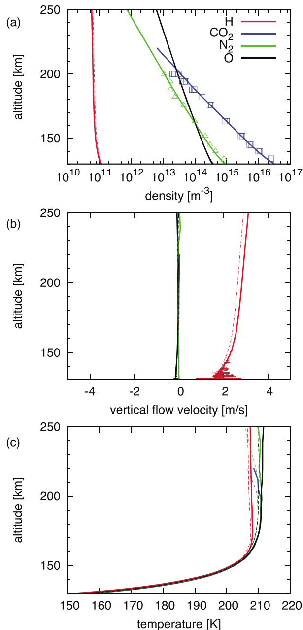
Figure 4. Altitude profiles of (a) densities, (b) vertical flow velocities, and (c) temperatures of H (red curve), CO 2 (blue curve), N 2 (green curve), and O (black curve) computed by the DSMC model for the 1 EUV case. The dashed curves show the results from the conventional model. The open squares and triangles in Figure 4a are the CO 2 and N 2 densities, respectively, measured by Viking 1 [Nier and McElroy, 1977].
