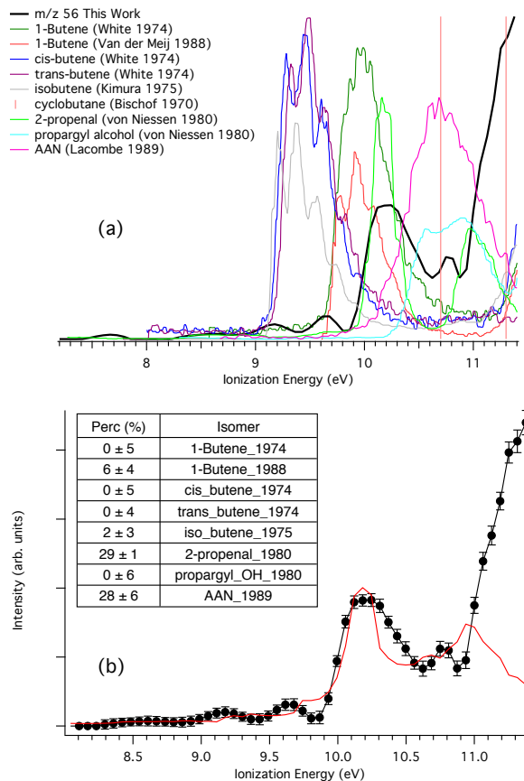
Figure 10: (a) Photoelectron spectrum for ion at m/z 56 obtained in this work at h\nu = 11.5 eV, along with those for the possible isomers found in the literature. 64-69 . The curves have been normalized to their integral over the displayed ionization energy range. (b) Experimental PES (black circles) and least squares fit of the linear combination of all isomers shown in panel (a) to the data. The contributions of each isomer to the data are shown in the inset.
