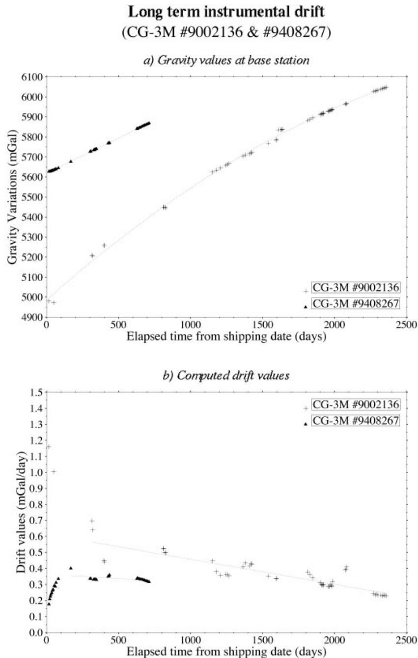
Figure 17. Long-term instrumental drift for the Scintrex CG-3M gravimeters. (a) Gravity field values measured at the reference site in Bondy with instruments 9002136 and 9408267 since their first use. The jump seen around day 1600 follows the opening of the sensor during a control by the manufacturer. (b) Corresponding instrumental drift values computed over continuous recording periods greater than or equal to three days.
