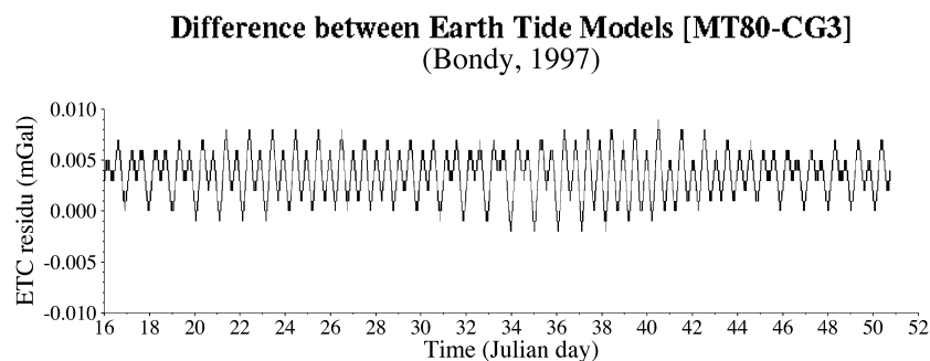
Figure 2. Difference between two theoretical models of the Earth tide between 01/16/97 and 02/20/97 at ORSTOM Research Centre in Bondy (48.915°N, 2.486°E). The residual signal is the difference between the correction computed by the Scintrex CG3 software [Longman (1959) algorithm] and the correction computed using the amplitude and phase coefficients determined by the Royal Observatory of Belgium (MT80 software).
