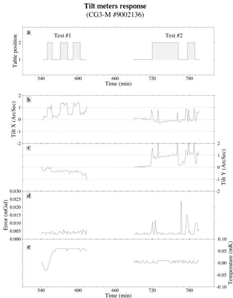
Figure 19. Results of an experimental test on the tilt response of the gravimeter 9002136 (sampling rate=1 reading per 90 sec). Curve a, tilts induced in the X axis (test 1) and the Y axis (test 2) of the gravimeter (see Fig. 18). In both tests, the calibration table was tilted alternately from position 1 (tilt=0) to position 2 (tilt= 4 \mu\text{rad} ). Curve b, tilt response of the gravity meter along the X axis. Curve c, tilt response of the gravity meter along the Y axis. Curve d, standard error of the gravity measurement series. Curve e, internal temperature of the gravimeter.
