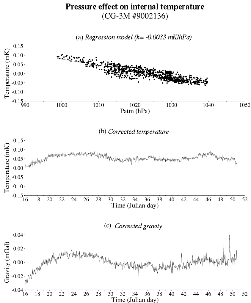
Figure 9. Influence of the atmospheric pressure on the internal temperature of the gravimeter 9002136 (see text and Figs 7 and 8). (a) Regression model between the two parameters. The corrected temperature (b) and gravity (c) signals should be compared to the raw data in Figs 8 and 5, respectively.
