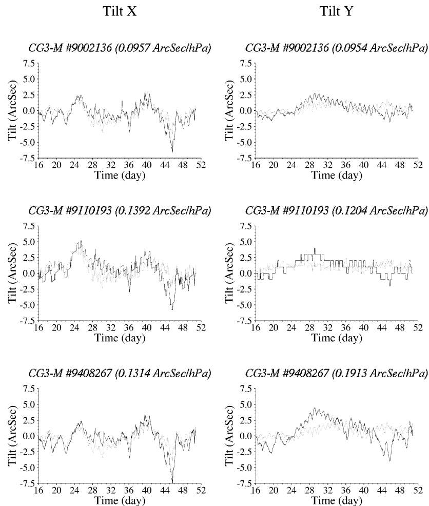
Figure 11. Influence of the atmospheric pressure on the gravimeter tilt-meter responses (Bondy, from 01/16/97 to 02/20/97). Thick lines show uncorrected tilts and thin lines show tilts corrected using the coefficient determined for each meter by a linear regression between the two parameters (see text and Table 1).
