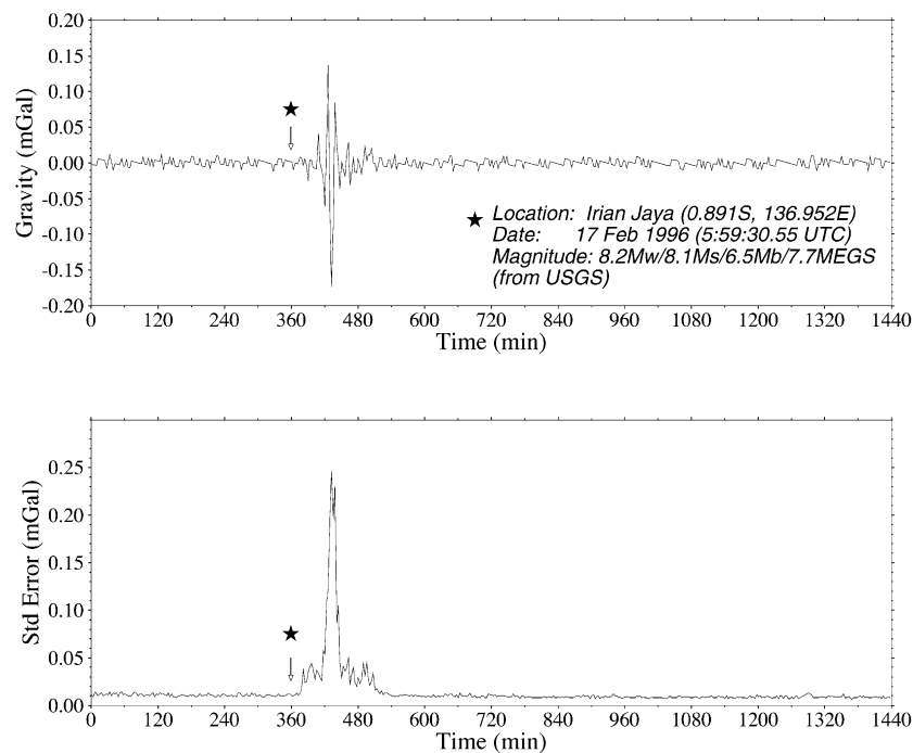
Figure 20. Response of gravimeter 9002136 to a teleseismic event with a large magnitude (8.2), recorded in Bondy ( 48.915^\circ\text{N} , 2.486^\circ\text{E} ). The residual gravity signal was obtained after removal of a precise Earth tide model and of a linear drift. It can be seen that no significant change occurs in the gravity response (drift value, accuracy) due to the recording of this perturbing signal. (a) Gravity response (sampling rate = 1 reading per 120 s). (b) Corresponding standard error in gravity measurements.
