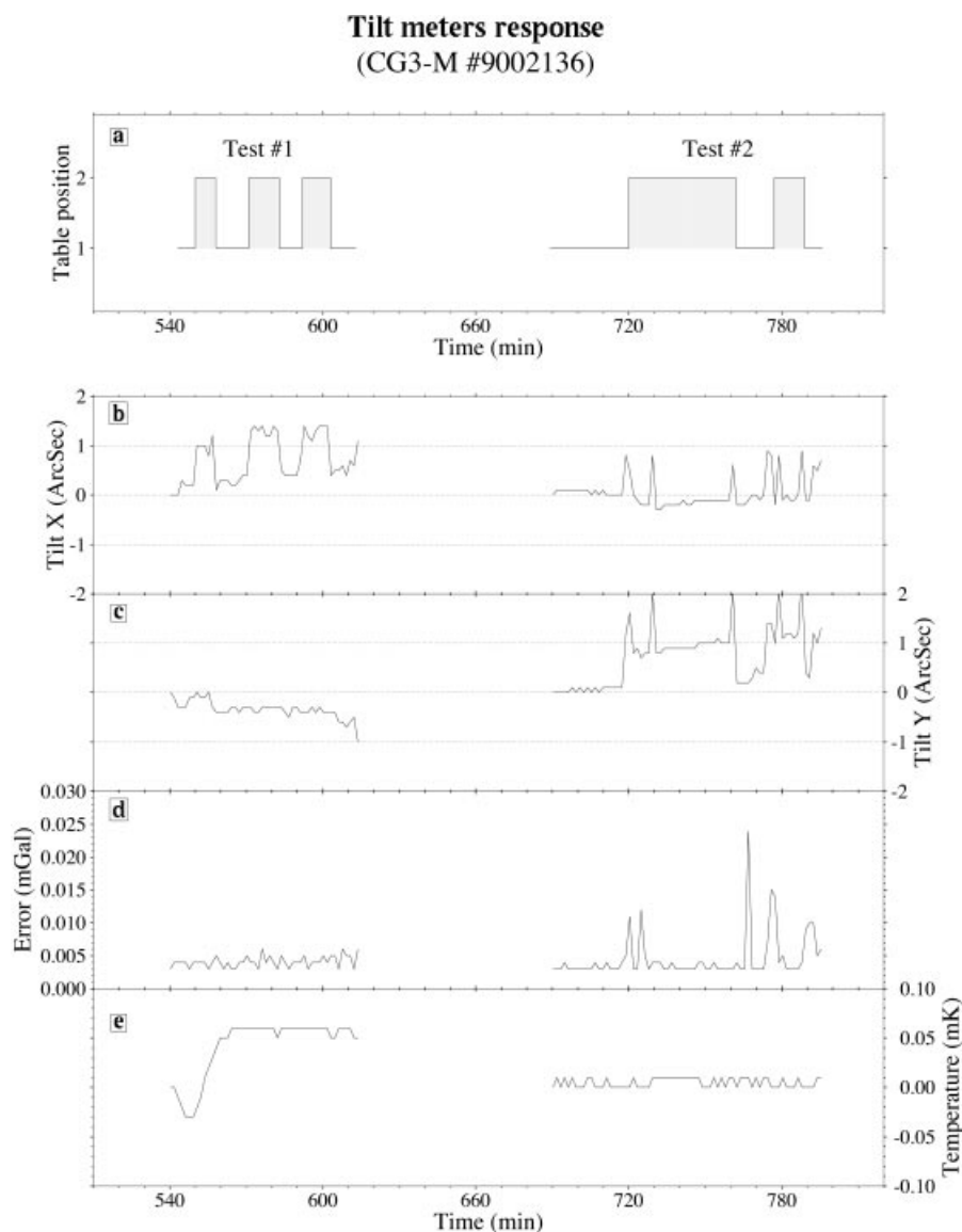
Figure 19. Results of an experimental test on the tilt response of the gravimeter 9002136 (sampling rate = 1 reading per 90 sec). Curve a, tilts induced in the X axis (test 1) and the Y axis (test 2) of the gravimeter (see Fig. 18). In both tests, the calibration table was tilted alternately from position 1 (tilt = 0) to position 2 (tilt = 4 \mu\text{rad} ). Curve b, tilt response of the gravity meter along the X axis. Curve c, tilt response of the gravity meter along the Y axis. Curve d, standard error of the gravity measurement series. Curve e, internal temperature of the gravimeter.
