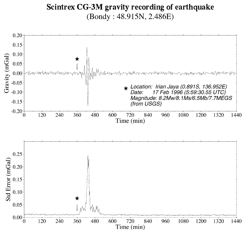
Figure 20. Response of gravimeter 9002136 to a teleseismic event with a large magnitude (8.2), recorded in Bondy ( 48.915^\circ\text{N} , 2.486^\circ\text{E} ). The residual gravity signal was obtained after removal of a precise Earth tide model and of a linear drift. It can be seen that no significant change occurs in the gravity response (drift value, accuracy) due to the recording of this perturbing signal. (a) Gravity response (sampling rate = 1 reading per 120 s). (b) Corresponding standard error in gravity measurements.
