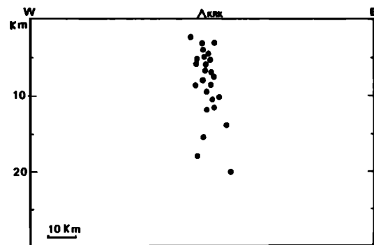
Fig. 8. East-west cross section across Krakatau.
