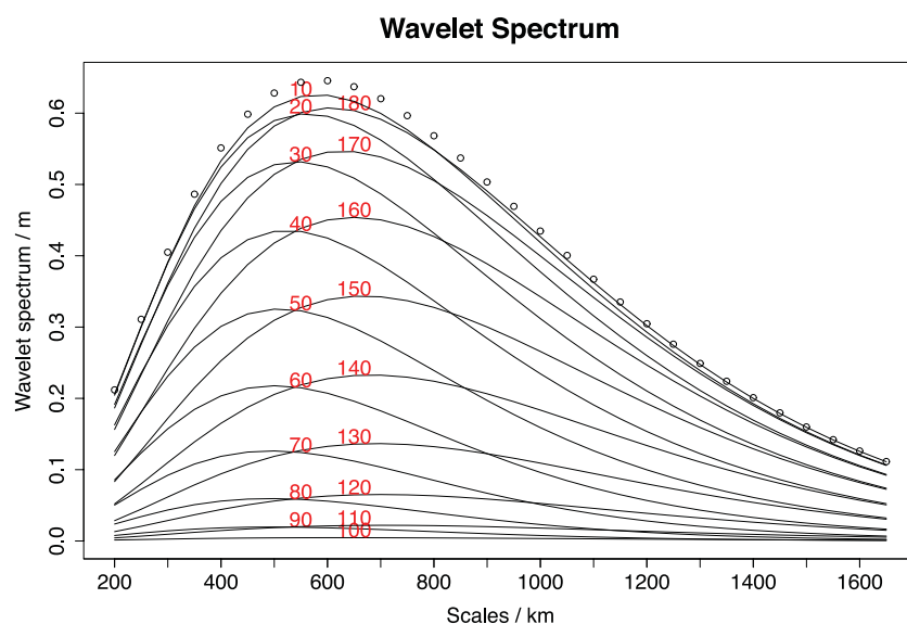
Figure 8. Directional wavelet spectra (in black solid lines) for the superposition of two synthetic signals of close scales (500 and 700 km) and close directions, for each investigated direction (noted in red). The spectrum for the dominant directions is given in circles. The direction difference is 10^\circ .
