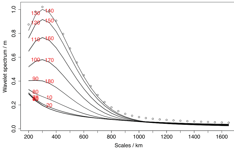
Figure 4. Directional wavelet spectra (in black solid lines) of a 300 km scale synthetic undulation superposed to Gaussian white noise, for each investigated direction (noted in red). The spectrum for the dominant directions is given in circles. The noise-to-signal amplitude ratio is 1:1.
