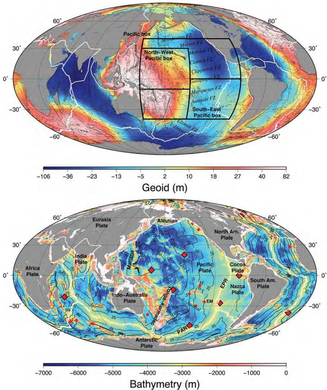
Figure 1. Top Panel: Map of the geoid anomalies of the world oceans computed from the EGM2008 model Pavlis et al. (2008) up to degree/order 360. The 1000 m contours of the GEBCO bathymetry are superimposed in black lines. The fracture zones of the Pacific ocean are indicated. The following abbreviations have been used: FZ: fracture zone, EM: easter microplate. The three areas (Pacific box, North-West Pacific box and South-East Pacific box) where the scaling properties of the geoid undulations are studied in Fig. 22 are delimited by red boxes. Bottom Panel: Map of the GEBCO bathymetry of the world oceans, with the tectonic plates limits and the major islands chains of the Pacific. The 25, 50, 75, 125, 150 and 175 M.y. isochrons of the ocean floor from Müller et al. (1997) are superimposed in black lines. Tectonic plate boundaries are indicated in white lines. Major and secondary hotspots are indicated in resp. large and small red diamonds. The following abbreviations have been used: EPR: East Pacific Rise, PAR: Pacific-Antarctic Ridge, EM: easter microplate, M: Marquesas islands, T: Tuamotu islands, S: society islands.
