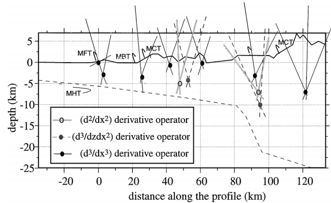
FIG. 12. Recapitulation of all the localizations of sources geometrically obtained along the Nepalese profile. Three different derivation operators of the real wavelet have been used. The black dashed line corresponds to the MHT flat-ramp-flat deep detachment (as inferred by active and passive seismological experiments).
