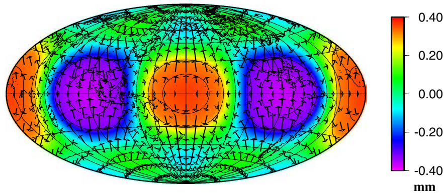
Figure 1. The perturbed M2 body-tide displacement due to ellipticity. The colour scale represents the vertical displacement in millimetres, and the arrows represent the perturbed tangential displacement (maximum of 0.3 mm), on the ellipsoid. The reference earth model is PREM.
