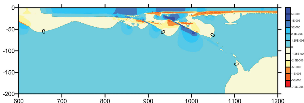
Figure 6. Accumulated dilatation 36 months after the main coseismic rupture. Density variation in the general part of the area below 50 km is positive, hence the resulting gravity anomaly at GRACE resolution is also positive.
