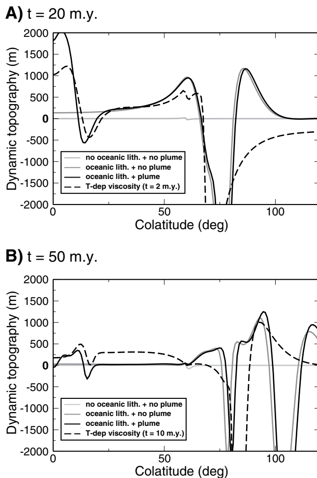
Figure 7. Dynamic topography as a function of colatitude for two snapshots at t = 20 m.y. (top panel) and t = 50 m.y. (bottom panel). Light-gray lines represent the case where the plume and dense oceanic lithosphere are not considered. Dark-gray lines represent the case where only the dense oceanic lithosphere is considered (i.e., no plume rise). Black lines represent the case where the dense oceanic lithosphere is considered along with a plume initiated by an ~40° lateral extension thermal anomaly at the core-mantle boundary. Black dashed lines represent the case in which temperature-dependent viscosity is implemented (with a viscosity of the coldest material 100 times larger than the viscosity of the hottest material).
