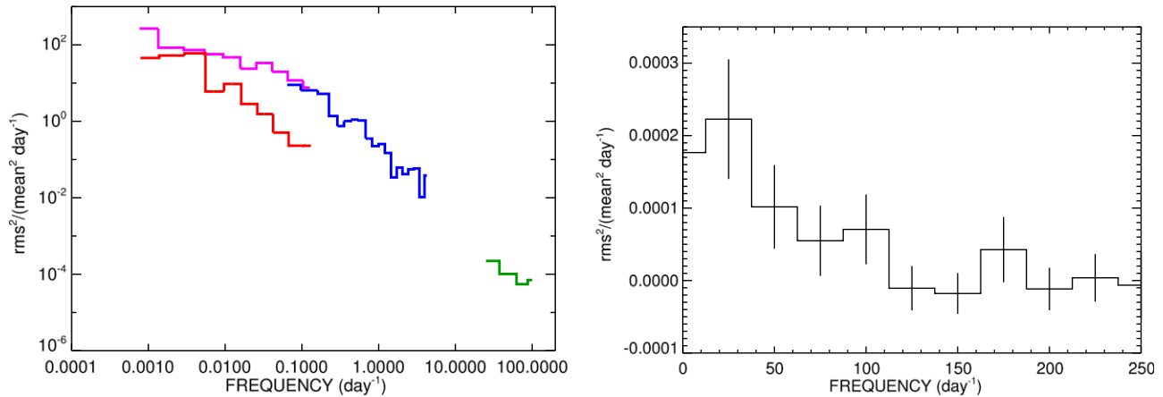
Figure 3. Power density spectrum (PDS) of the \gamma -ray flux of 3C 279. (left) PDS derived from three different time-binned light curves: 3 days (red and magenta), orbital period (blue), and 3 minutes (green). The PDSs marked in red and magenta were derived using the first and second halves of the first 7 year Fermi -LAT observation, respectively. The second half of the interval contains the giant outburst phase in 2015 June. (right) Enlarged view of the high-frequency part of the PDS, based on 3-minute binned light curves, plotted using a linear scale and also including the highest frequencies. The white noise level has been subtracted.
