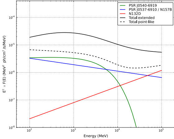
Fig. 8. Comparison of the total emission of extended nature with that of point sources for which an established or likely association with an LMC object exists (as indicated in the legend). Best-fit analytic spectra were used and summed over components E0 to E4 to produce the black curve for the diffuse contribution.
