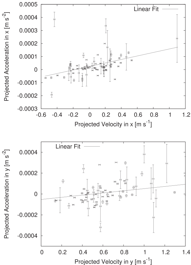
Figure 7. Correlation between acceleration and velocity, for the horizontal (top) and vertical (bottom) components. The solid lines represent linear fits with a_x = 1.3 \times 10^{-4} \text{ s}^{-1} v_x + 0.2 \times 10^{-4} \text{ m s}^{-1} and a_y = 10^{-4} \text{ s}^{-1} v_y - 0.5 \times 10^{-4} \text{ m s}^{-1} .
