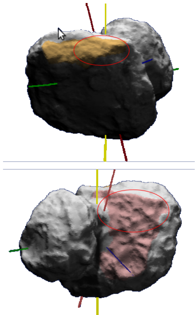
Figure 12. The nucleus of 67P as seen from Rosetta at the time of our observations (top panel) with the Khonsu region in colour, and (bottom) as an observer on the other side of the nucleus would have seen it with the Seth region coloured. The red ellipses roughly indicate the locations of our inferred source regions. The yellow line indicates the Sun–comet line, and the green, red, and blue lines represent the x -, y -, and z -axes in the standard reference frame of the comet. The z -axis coincides with the comet’s rotation axis. The upper panel includes the South pole at the right edge of the big lobe, and the centre of the lower panel shows the North pole. The images were generated with the CG viewer tool of the OSIRIS team developed by Tim Wittrock at https://planetgate.mps.mpg.de:8114 .
