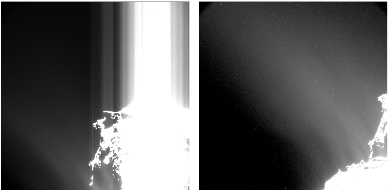
Figure 5. NAVCAM images acquired at 12:29 (left) and 12:55 (right). The first image was taken without attenuation filter and 0.01 s exposure time. The vertical structures towards the top right are blooming artefacts due to saturation on parts of the nucleus. The second image is part of a navigation raster with attenuation filter and 1.75 s exposure time. The grey-scales were adapted such that the maximum (white colour) corresponds to 1 \times 10^{-4} \text{ W m}^{-2} \text{ sr}^{-1} \text{ nm}^{-1} .
