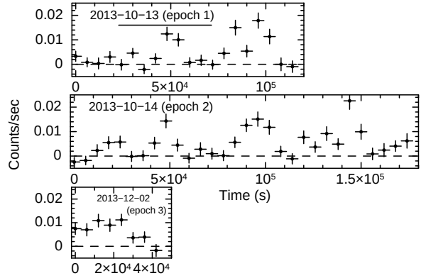
Fig. 2.— NuSTAR FPMA light curves for three epochs of observations in the 3–25 keV energy band with 6000 s time binning. The solid horizontal line in the top panel indicates the time of the XMM-Newton observation.
