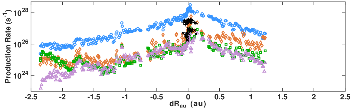
Figure 11. Evolution of the production rate for the species H 2 O (blue), CO 2 (orange), CO (green), and O 2 (purple) from the DFMS data using the DSMC model to take into account the asymmetry of the coma and the evolution of the velocity as a function of heliocentric distance with respect to the closest approach (1.24 au) dR_{\text{au}} using the definition that dR_{\text{au}} is negative before perihelion and positive after perihelion. The black plus and cross symbols represent, respectively, the H 2 O and CO 2 production rates deduced from the VIRTIS-H observations using the DSMC model.
