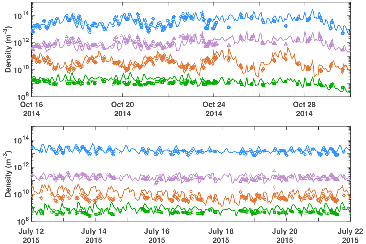
Figure 8. Diurnal evolution of the number density for \text{H}_2\text{O} (blue), \text{CO}_2 (orange), \text{CO} (green), and \text{O}_2 (purple) from the ROSINA data (symbols) compared with the DSMC model (solid lines). To clarify the plot and avoid overlapping, the \text{CO}_2 densities were divided by factors of 20 and 200, and \text{CO} by factors of 400 and 3000 in the top and lower panels, respectively.
