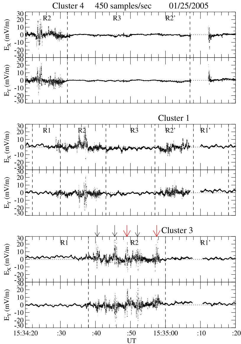
Figure 9. Electric field measurements from the EFW instrument showing two spin-plane component (X, Y ~GSE) measurements from the double probe instrument on C4, C1, and C3. The temporal resolution is 450 Hz. The region boundaries are set by the FGM and CIS data, as described in the text. Arrowed in the bottom plot are the discrete bursts of enhanced electric field activity.
