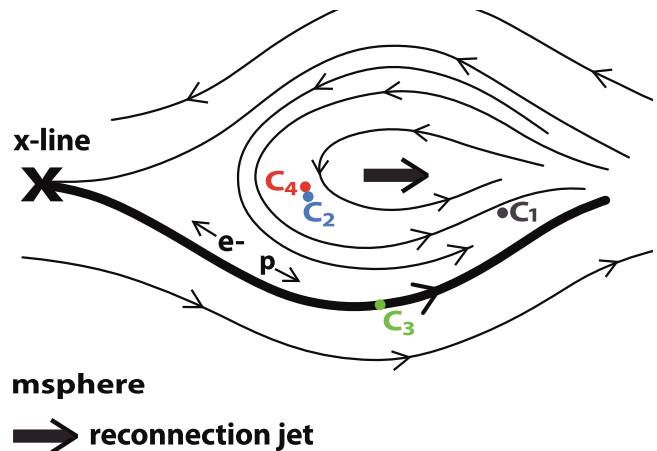
Figure 16. A sketch of the magnetic field configuration at the time when Cluster 3 is observing one of the discrete burst of large-amplitude electric field fluctuations. For further details, see text.
