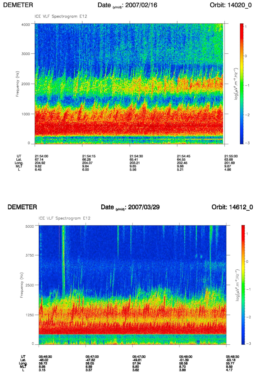
Figure 3. (top) Spectrogram up to 4 kHz of an electric component registered on 16 February 2007 between 21:54:00 and 21:55:00 UT. (bottom) Spectrogram up to 5 kHz of an electric component registered on 29 March 2007 between 05:46:30 and 05:48:30 UT. The intensities of the spectrograms are color coded in accordance with the scales on the right. The parameters presented below are the time in UT, the geographic latitude and longitude, the magnetic local time, and the McIlwain parameter L .
