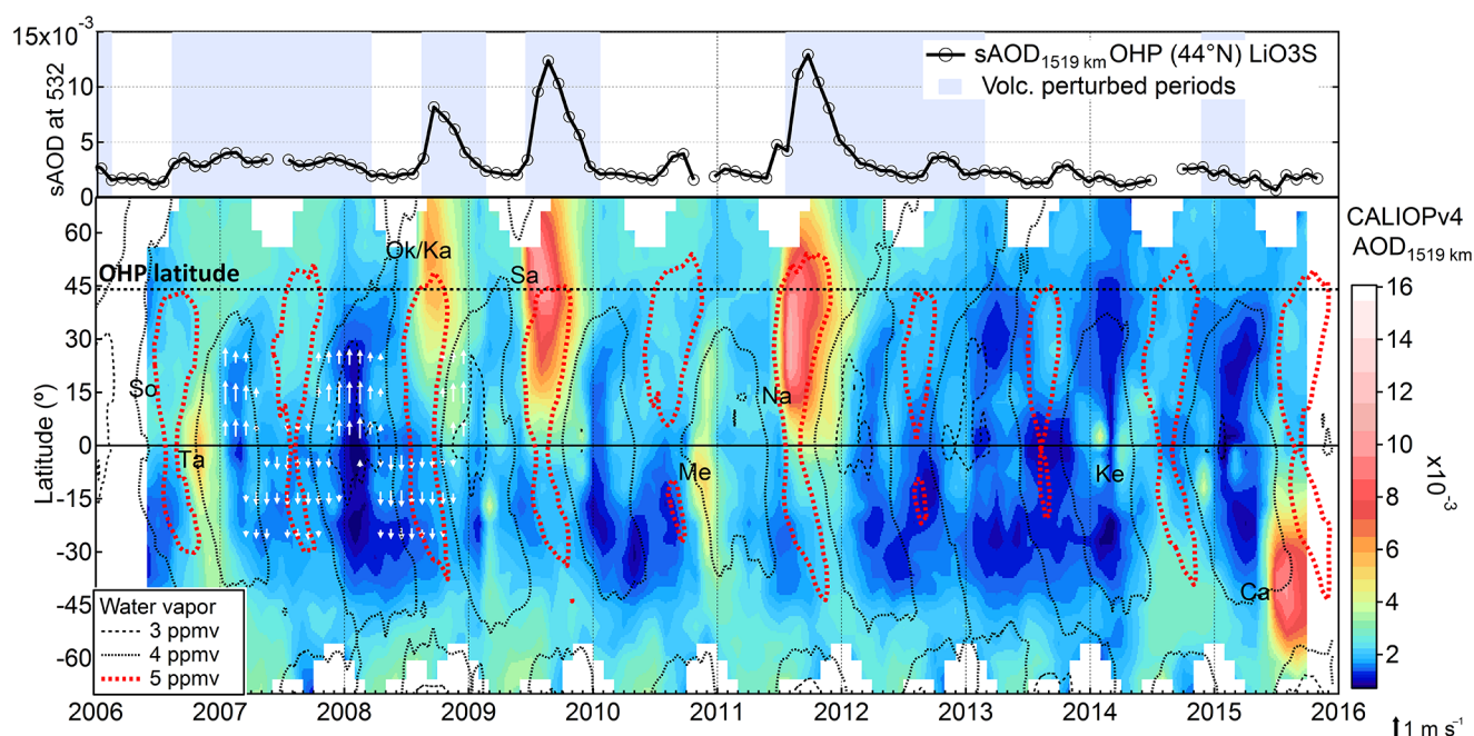
Figure 6. Time series of monthly mean sAOD_{1519} from OHP LiO3S lidar (top) and time–latitude section of zonal-mean AOD_{1519} from CALIOP in log-scaled color map with indications of VEI 4 eruptions (bottom). Time periods considered as perturbed by volcanism (Table 3) are shaded light blue in the top panel. White arrows (in 2007–2008) represent the mean meridional component of monthly and zonally averaged horizontal wind at 100 hPa from ERA-Interim reanalysis. Dashed and dotted contours depict the zonal-mean water vapor mixing ratio at 100 hPa from Aura MLS.
