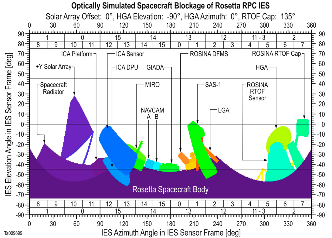
Figure 1. A simulation showing known objects with IES' field of view [Acton, 1996]. The azimuthal ranges of IES' ion and electron anodes are marked above and below the figure, respectively, as the outer and inner labels.
