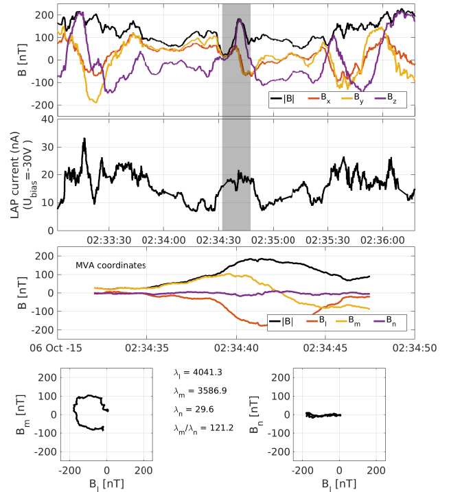
Figure 8. Results from an MVA analysis of one identified flux rope. The top panel shows the MAG data in CSEQ coordinates with the grey shaded region indicating the flux rope. The second panel shows the LAP1 ion current, which is proportional to ion density. The third panel shows the MVA coordinates from the time indicated by the grey shaded region, and the lower two panels show hodograms of the magnetic field components in MVA-coordinates. The eigenvalues as well as the ratio between the eigenvalues associated with the intermediate and the minimum components are also stated.
