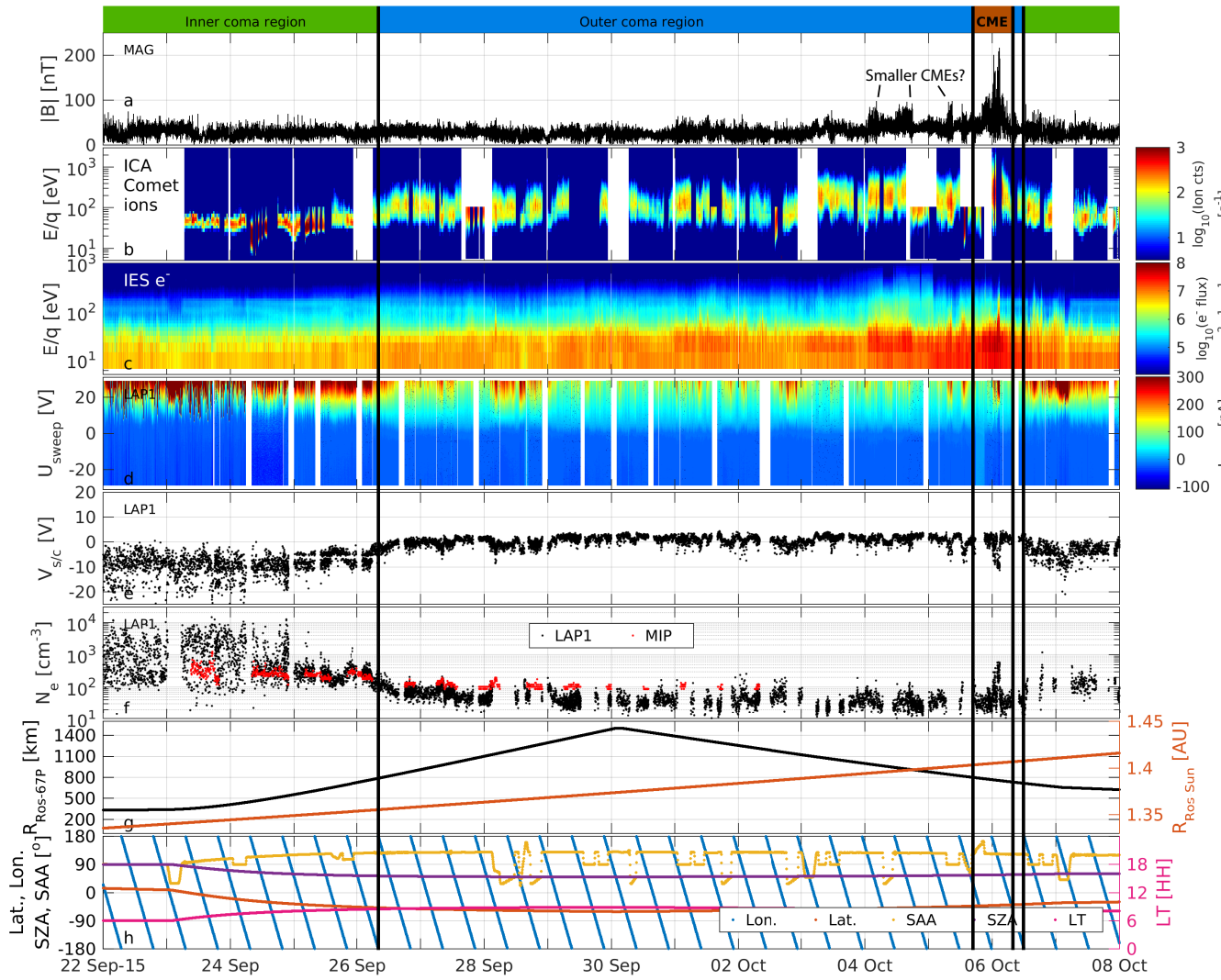
Figure 3. Overview of RPC data from the dayside excursion and especially including the interval of the CME impact. The panels show (a) the magnetic field strength, (b) spectrogram of ICA measured heavy (cometary) ions, (c) spectrogram of IES measured electrons (d) LAP sweeps (current collected is colour-coded, bias potential fed to the probe on the vertical axis) (e) spacecraft potential measured by LAP (f) electron density measured by LAP (black dots) where data points during spacecraft attitude changes are excluded together with MIP density estimates (red dots), (g) distance to the comet and the Sun from Rosetta (h) longitude and latitude (projected down on a sphere), SZA, SAA (attitude angle) and Local time (LT) of Rosetta.
