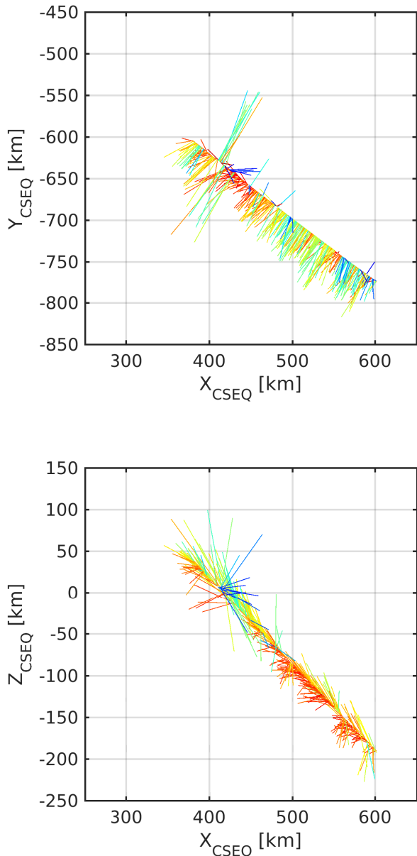
Figure 11. Magnetic field vectors projected on to the (top) x - y plane and (bottom) x - z plane along the Rosetta trajectory from 00:00 UT 4 Oct 2015 until 12:00 UT 6 Oct 2015. Red colours indicate an out-of-plane component, blue and in-to-plane component and green in-plane. The magnetic field is mainly directed in the -x , -y -direction before the large field rotations on 6 Oct 2015.
