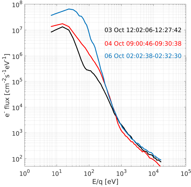
Figure 5. IES electron energy spectra during three intervals before and during the CME impact. Up to an order of 10 increase in electron fluxes for energies below 200 eV during the CME impact are observed during the CME impact (blue and red line), compared to before (black line).
