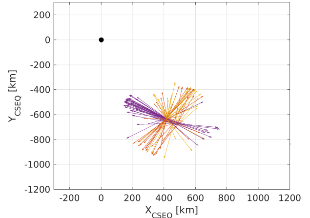
Figure 10. MVA vectors of 40 identified events in the interval 4 Oct 2015 - 6 Oct 2015. The purple vectors show the minimum variance direction, which are aligned with the rope axis. The red and the orange arrows indicate the maximum and intermediate variance direction, respectively. The 40 ropes all have very similar orientation and are directed slightly off the direction to the nucleus at (x,y)=(0,0)
