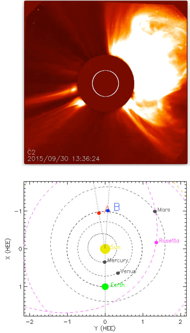
Figure 2. (Top) SOHO LASCO2 image of a CME being released on 30 Sep 2015 in the general direction of Rosetta (Image from http://sohowww.nascom.nasa.gov/data/realtime/ ). (Bottom) Position of the inner planets and Rosetta on 30 Sep 2015. A and B indicate the positions of the Stereo-A and Stereo-B spacecraft, which did not observe the CME. There were unfortunately no spacecraft in operation at Mercury or Venus. At Mars, both the MAVEN and the MEX spacecraft were measuring the solar wind intermittently and saw a weaker signature of the CME (Figure from http://stereo-ssc.nascom.nasa.gov/cgi-bin/make_where_gif ).
