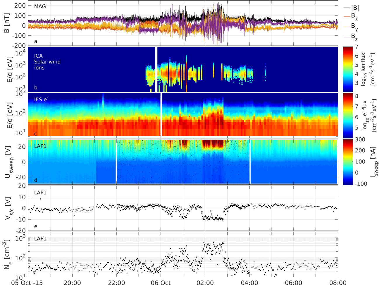
Figure 4. Time series of RPC data covering the interval of the CME impact. The panels show (a) magnetic field magnitude and components in CSEQ coordinates, (b) spectrogram of solar wind ions (c) spectrogram of electron fluxes (d) Langmuir probe sweeps, (e) spacecraft potential, and (f) electron density derived from the Langmuir probe sweeps.
