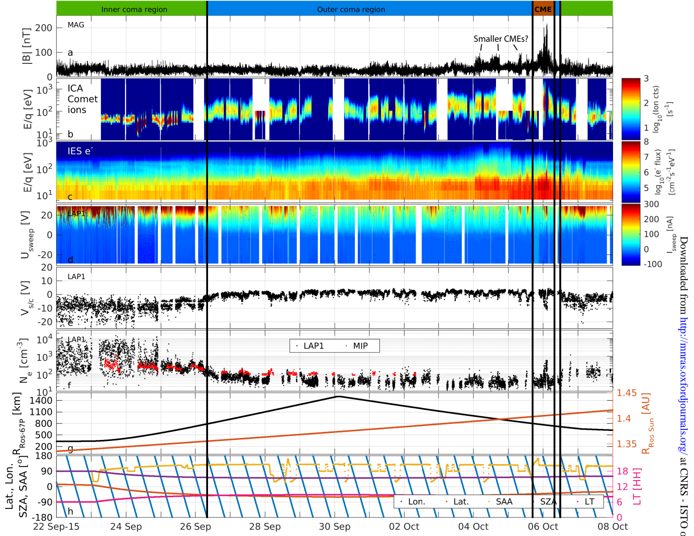
Figure 3. Overview of RPC data from the dayside excursion and especially including the interval of the CME impact. The panels show (a) the magnetic field strength, (b) spectrogram of ICA measured heavy (cometary) ions, (c) spectrogram of IES measured electrons (d) LAP sweeps (current collected is colour-coded, bias potential fed to the probe on the vertical axis) (e) spacecraft potential measured by LAP (f) electron density measured by LAP (black dots) where data points during spacecraft attitude changes are excluded together with MIP density estimates (red dots), (g) distance to the comet and the Sun from Rosetta (h) longitude and latitude (projected down on a sphere), SZA, SAA (attitude angle) and Local time (LT) of Rosetta.
