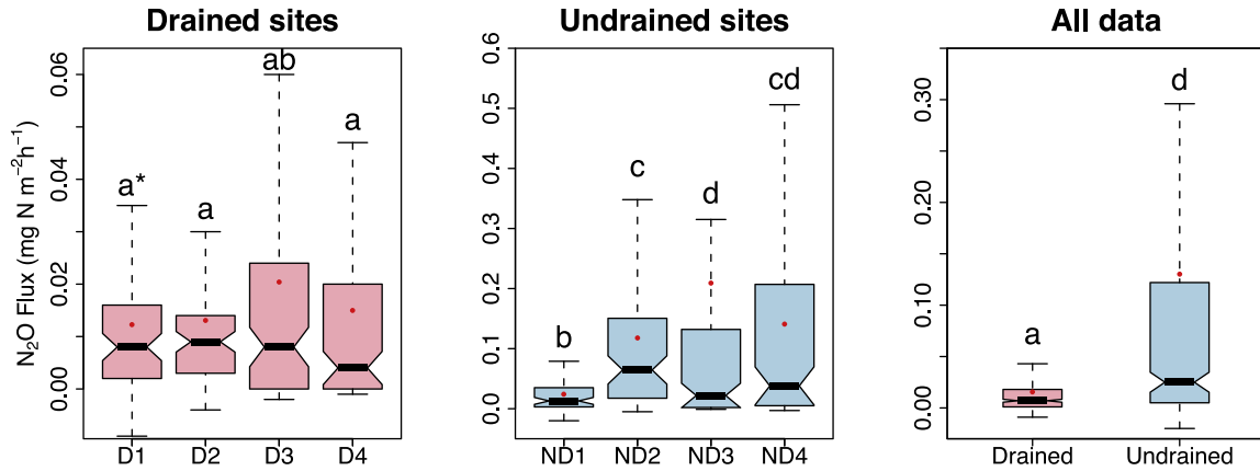
Fig. 3. Box plot of N_2O fluxes for drained sites (left), undrained sites (middle) and merged data from all sites (right). The point indicates the mean value. The letter above boxes indicates whether flux distribution was significantly different at the 0.05 level with a Mann-Whitney test.
