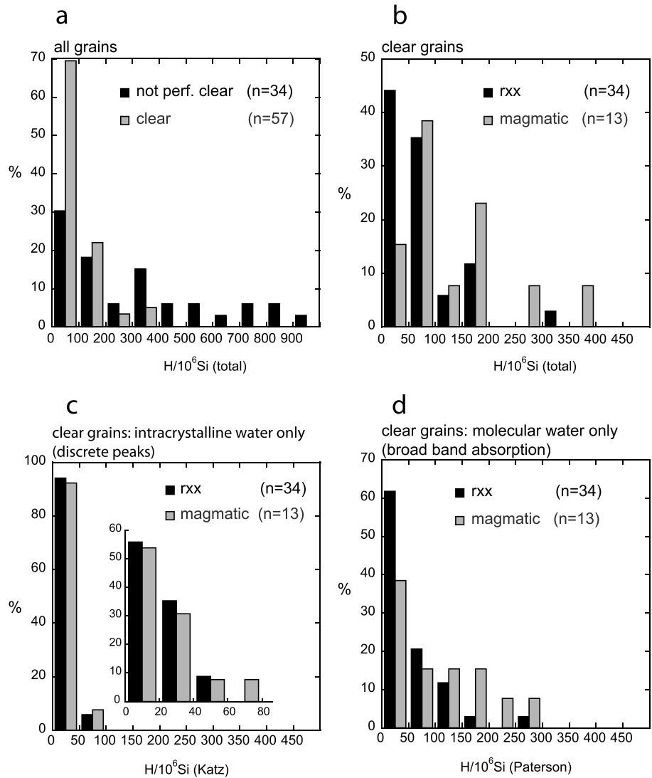
Figure 11. Quantification of water content: (a) Histograms of the total water content calculated as the sum of molecular water (broad absorbance band using the calibration of Paterson [1982]) and H/OH species (discrete peaks, using the calibration of Katz [1962]) for clear and not perfectly clear grains. (b) Histogram of quantities for recrystallized (rxx) and magmatic, clear grains. Grain populations are the same as used in Figure 10. (c) Histogram of intracrystalline water content in magmatic and recrystallized, clear grains; inset shows the data for narrower bins. (d) Histogram of the molecular water content in magmatic and recrystallized grains. Units are given in H/10^6 Si .
