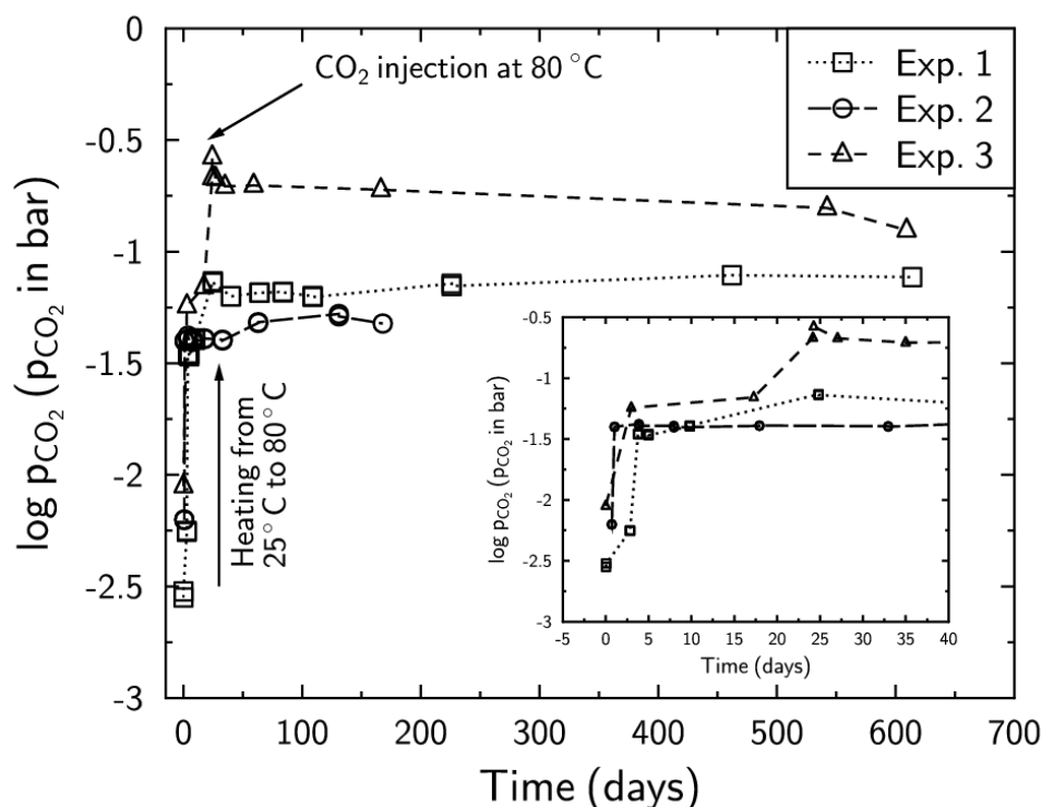
Fig. 2. Evolution of the partial pressure of CO_2 (in bar) as a function of time for the experiments at 80^\circ C in reactors. The initial p_{CO_2} correspond to the p_{CO_2} at near-equilibrium with the water/clay-rock system at
