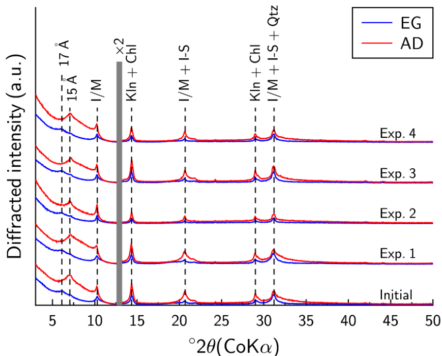
Fig. 4. Experimental XRD patterns (oriented slides, decarbonated and Ca-saturated < 2 \mu\text{m} size fraction) of the initial sample and of the samples reacted at 80 \text{ }^\circ\text{C} . The red and blue solid lines represent patterns recorded in the air-dried (AD) state and after ethylene glycol (EG) solvation, respectively. Peak positions are outlined as dashed lines for illite/mica (I/M), chlorite (Chl), kaolinite (Kln), mixed-layer illite/smectite (I-S) and quartz (Qtz) contributions. The vertical gray bars indicate a modified scale factor for the high-angle regions compared to the 2\text{-}13^\circ 2\theta angular range. XRD intensities were normalized from I/M intensity at 10.2^\circ 2\theta .
