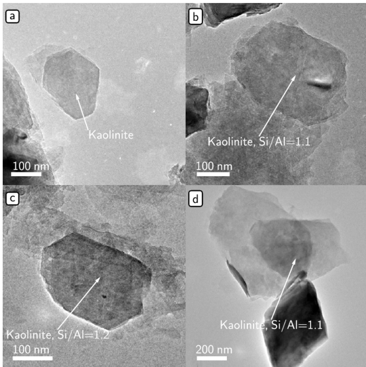
Fig. 7 . TEM micrographs of kaolinite in the samples: (a) and (b) thin particles observed in the initial clay-rock sample; (c) and (d) particles in the samples reacted at 80 °C for 20 months in an anoxic atmosphere.
