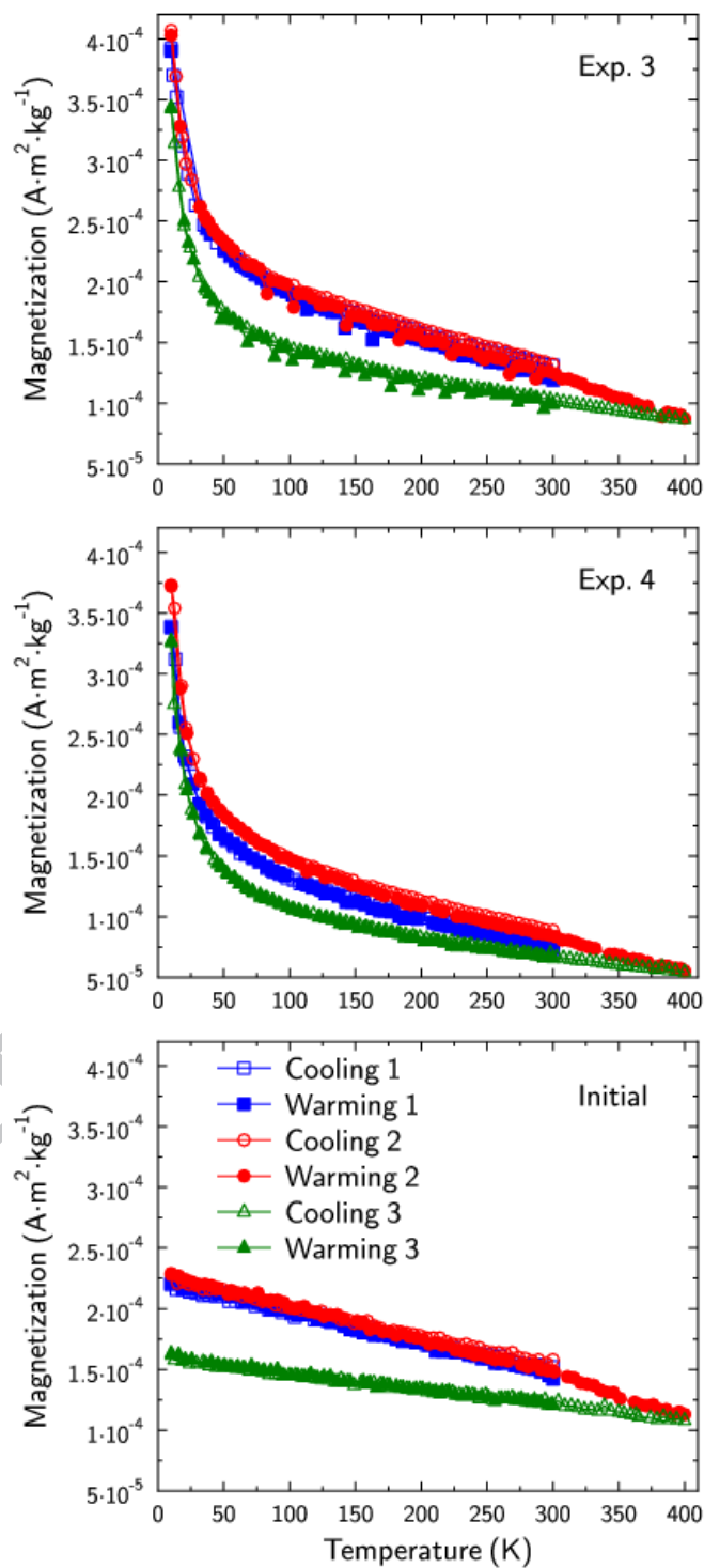
Fig. 9. Evolution of the room temperature saturation isothermal remanent magnetization for the two final samples from experiments 3 and 4, compared to initial sample (Kars et al., 2015) during
