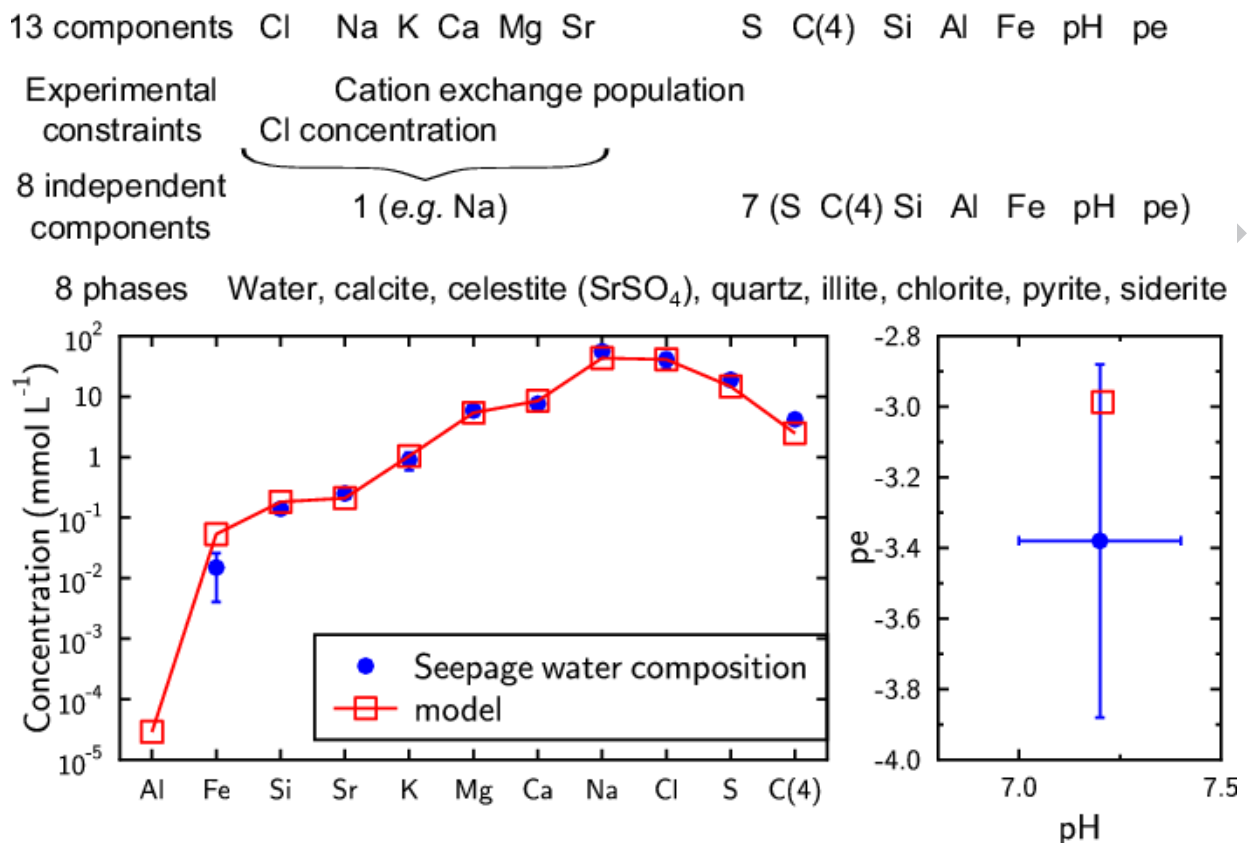
Fig. 1. Top: the fully constrained pore water model for the system pH, pe, Cl, S, Na, K, Ca, Mg, Sr, C(4), Si, Al, Fe in the Callovian-Oxfordian clay-rock (Bure, France) at 25 °C. Bottom: corresponding predicted pore water composition as compared to seepage water composition. Reproduced from Tournassat et al. (2015).
