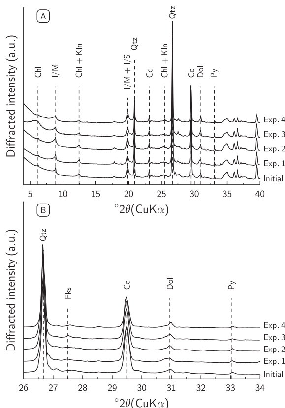
Fig. 3. Experimental XRD patterns on Callovian-Oxfordian powder samples acquired on the initial sample and on the samples reacted at 80 °C (a) between 4 and 40° 2θ and (b) zoom between 26 and 34° 2θ. Peak positions are outlined as dashed lines for illite/mica (I/M), chlorite (Chl), kaolinite (Kln), mixed-layer illite/smectite (I-S), quartz (Qtz), K-feldspar (Kfs), calcite (Cc), dolomite (Dol) and pyrite (Py).
