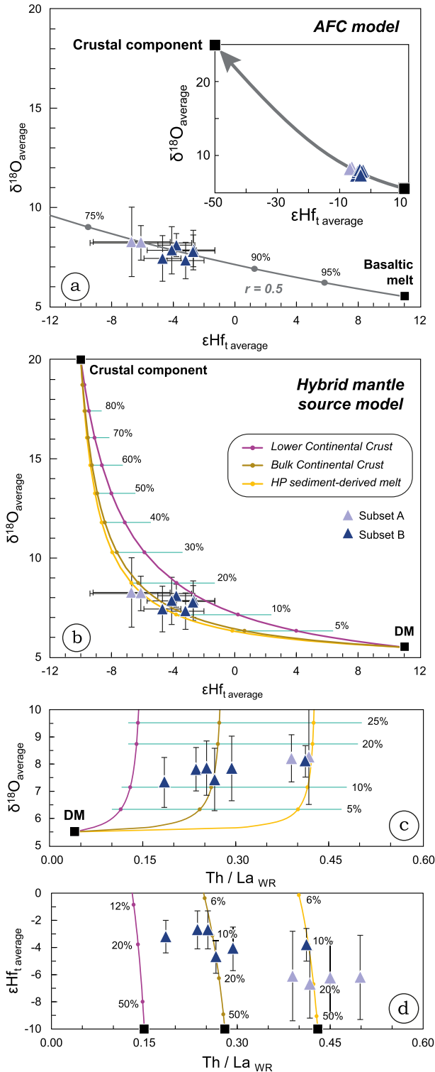
Fig. 6. (a) Results of assimilation/fractional crystallization (AFC) model of a basaltic melt (Hf content of 2.03 ppm, from Sun and McDonough, 1989; DM-like isotopic composition with \epsilon\text{Hf}_t = +11 calculated from Naeraa et al., 2012, and \delta^{18}\text{O} = +5.3 from Valley et al., 1998) assimilating bulk continental crust (Hf content of 3.7 ppm, from Rudnick and Gao (2003); \epsilon\text{Hf}_t = -50 and \delta^{18}\text{O} = +25 adjusted to fit the data for a maximum fractionation rate of ca. 20%); grey dots indicate the fraction of remaining liquid and r the mass ratio between assimilated and crystallized material. (b), (c) and (d) Results of mass-balance, binary mixing models between DM ( \epsilon\text{Hf}_t = +11 ; \delta^{18}\text{O} = +5.3 ; Hf contents [0.2 ppm] and Th/La [0.04] from Workman and Hart (2005)) and three different crustal materials, all characterized by \epsilon\text{Hf}_t = -10 and \delta^{18}\text{O} = +20 (adjusted to fit the data for a maximum mantle contamination rate of ca. 20%): (i) a melt derived from HP melting of terrigenous sediment (Hf contents [4.3 ppm] and Th/La [0.43] from Plank and Langmuir, 1998, corrected from HP melting using average partition coefficients of Hermann and Rubatto (2009)); (ii) Lower and (iii) Bulk Continental Crust (Rudnick and Gao, 2003). O contents are from Roberts et al. (2012). Light blue lines denote the percentage of crustal component in the mixture. Error bars for samples are 2 S.D. All \epsilon\text{Hf}_t are calculated at 310 Ma (average age of PCMM in the eastern FMC). (For interpretation of the references to color in this figure legend, the reader is referred to the web version of this article.)
