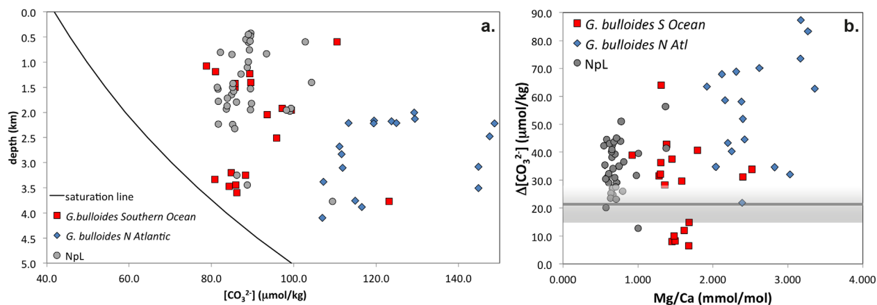
Figure 3. (a) Carbonate ion concentration ( [CO_3^{2-}] , \mu\text{mol/kg} ) at each station versus depth (km). The black line shows the calcite saturation line calculated using the [CO_3^{2-}]_{\text{sat}} equation of Bassinot et al. [2004]. (b) Degree of calcite saturation ( \Delta[CO_3^{2-}] , \mu\text{mol/kg} ) versus measured foraminiferal Mg/Ca (mmol/mol). Grey horizontal line and shadow shows the critical threshold of \Delta[CO_3^{2-}] = 21.3 \pm 6.6 \mu\text{mol/kg} defined by Regenberg et al. [2014]. Red squares: Southern Ocean G. bulloides sites; blue diamonds: North Atlantic G. bulloides sites; grey circles: Southern Ocean N. pachyderma left sites. Correlation coefficients for (b) R^2 = 0.13 for North Atlantic G. bulloides samples; 0.02 for Southern Ocean G. bulloides samples; 0.06 for N. pachyderma left samples.
