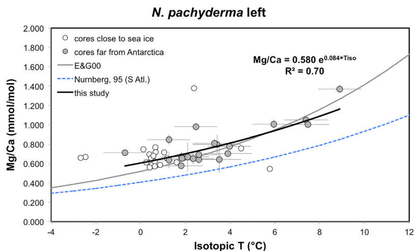
Figure 6. Mg/Ca (mmol/mol) versus isotopic temperature ( ^{\circ}\text{C} ) for N. pachyderma left. Circles are site averages, grey for sites north of 60^{\circ}\text{S} and away from the influence of sea ice, and white for sites close to the Antarctic margin. Black line indicates the exponential regression including sites not affected by sea ice (grey circles, equation (5)). The regression curves of Nürnberg [1995] (South Atlantic N. pachyderma left, blue dashed line) and Elderfield and Ganssen [2000] (multispecies, grey line) are also shown for comparison.
