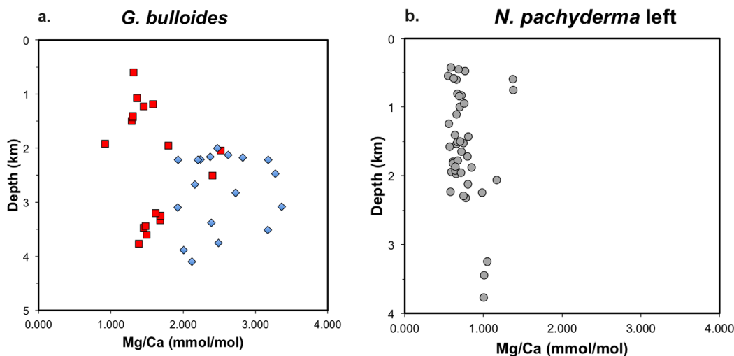
Figure 2. Variation of foraminiferal Mg/Ca (mmol/mol) with water depth (km) of the core tops. (a) G. bulloides samples. Red squares: Southern Ocean sites ( R^2 = 0.03 ); blue diamonds: North Atlantic sites ( R^2 = 0.01 ). (b) N. pachyderma left samples ( R^2 = 0.05 ).
