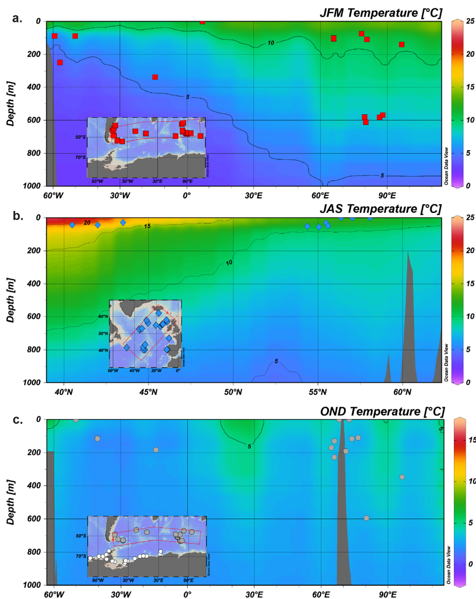
Figure 8. Calcification depths reconstructed from Mg/Ca-derived temperatures plotted over WOA09 temperature sections defined by red sections in the insets. (a) Summer (JFM) temperature meridional transect with Southern Ocean G. bulloides sites (red squares). (b) Summer (JAS) temperature latitudinal transect with North Atlantic G. bulloides sites (blue diamonds). (c) Spring (OND) temperature meridional transect with N. pachyderma left sites away from the influence of sea ice (grey circles). Also shown in the inset are N. pachyderma left sites affected by sea ice (white circles).
