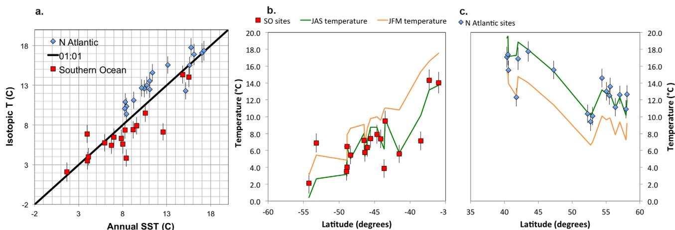
Figure 7. (a) Isotopic temperature of G. bulloides (°C) versus annual SST (°C) of the upper 50 m of the water column extracted from WOA09 [Locarnini et al., 2010] at the location of the North Atlantic and Southern Ocean sites. Black line indicates 1:1 relation. (b and c) Isotopic temperature of G. bulloides (°C) versus latitude of the core top sites in the Southern Ocean (b) and the North Atlantic (c). Orange line is January–March (JFM) temperature; green line is July–September temperature (JAS) from the WOA09 [Locarnini et al., 2010]. Red squares are sites located in the Southern Ocean and blue diamonds are sites in the North Atlantic.
