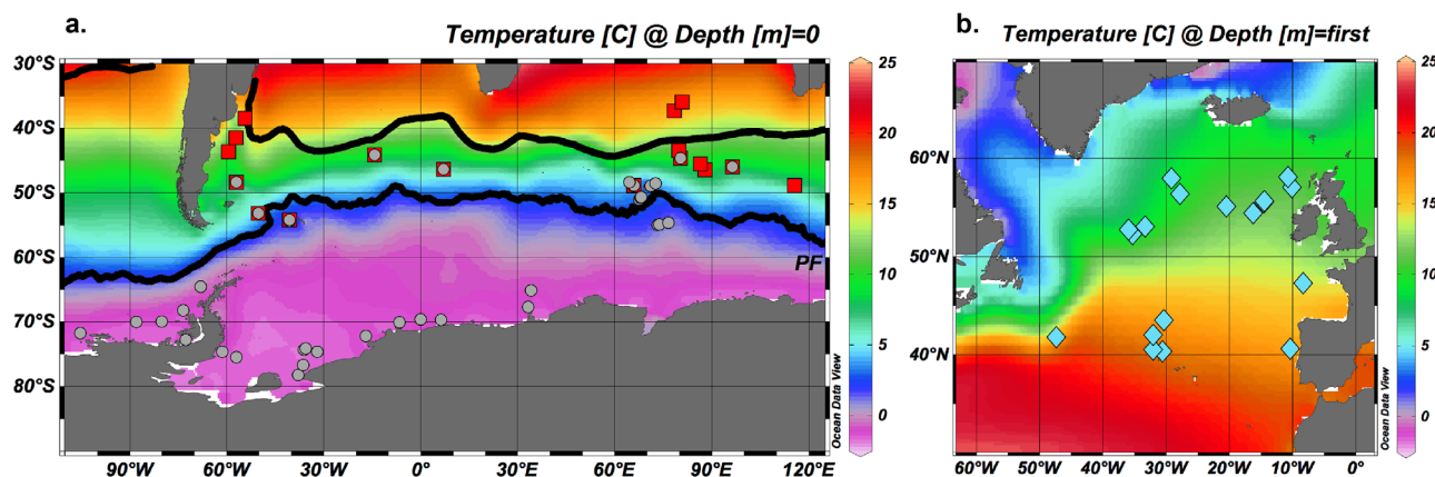
Figure 1. Maps showing core top locations and mean annual SST from the World Ocean Atlas 2009 [Locarnini et al. , 2010]. (a) Southern Ocean sites. Red squares indicate core top samples with G. bulloides ; grey circles indicate samples with N. pachyderma left. The black lines indicate the positions of the Polar Front (PF) and the Subtropical Front (STF) [Orsi et al. , 1995]. (b) North Atlantic sites. Blue diamonds indicate samples with G. bulloides [Bouinot, 2011; Cl  roux et al. , 2008].
