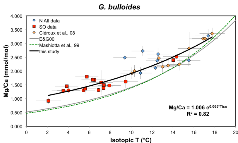
Figure 5. Mg/Ca (mmol/mol) versus isotopic temperature (°C) for G. bulloides . All symbols are site averages; red squares are new Southern Ocean data; blue diamonds are new North Atlantic data presented in this study [Bouinot, 2011]; orange diamonds are the data set of Cléroux et al. [2008] with T_{iso} recalculated as explained in section 2.4. Black thick line indicates the regression including all sites (equation (4)). The regression curves of Mashiotta et al. [1999] ( G. bulloides , green-dashed line) and Elderfield and Ganssen [2000] (multispecies, grey line) are also shown for comparison.
