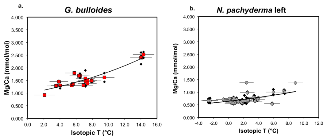
Figure 4. Mg/Ca (mmol/mol) versus isotopic temperature ( ^{\circ}\text{C} ). (a) G. bulloides Southern Ocean data. Red squares are site averages and black diamonds are replicas. Black thick line indicates exponential regression computed on averaged values of all Southern Ocean sites (equation (2), R^2 = 0.75 ). (b) N. pachyderma left data. Grey circles are site averages and black diamonds are replicas. Black thick line indicates the exponential regression computed on averaged values at all sites (equation (3), R^2 = 0.35 ). Error bars in both graphs are 1\sigma uncertainties in T_{\text{iso}} .
