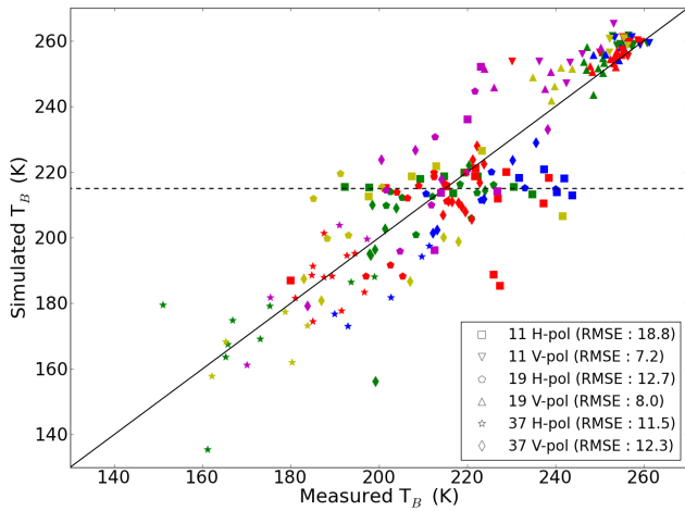
Figure 6. T_B simulated with ice lenses included in DMRT-ML but without bridging. The symbol types correspond to the frequency and colors to the sites: red is JB_{Jan} -transect; green is JB_{Jan} -others; blue is JB_{Feb} ; yellow is JB_{Mar} ; magenta is UMI. The dotted black line represents the T_B where the simulations underestimated the spatial variability at 11 and 19 GHz H-pol.
