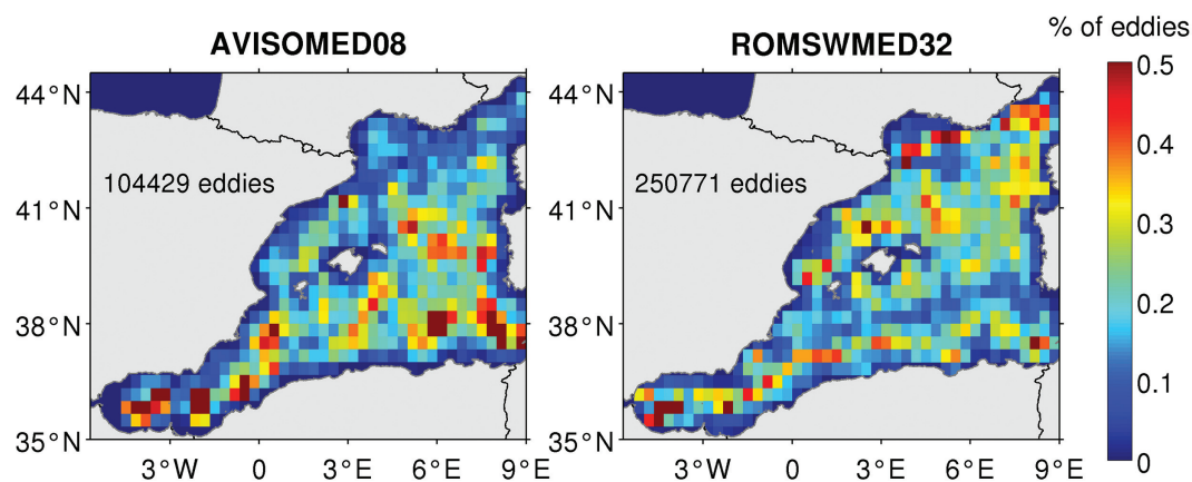
Figure 9. Percentage of detected eddies in each cell of 1/3° × 1/3° of the domain for both data sets. Each eddy is counted in the cell that contains its centroid on each day it is detected.
