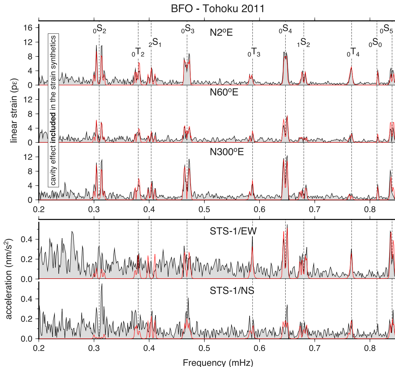
Figure 5. Same as Fig. 4 after the Tohoku quake. Time-series start at 6:45:00.0 UTC on 2011 March 11. The calibrated pressure was multiplied by the factors given in Table 1 and subtracted from the strain records and accelerograms. In addition, the Hilbert transform of the pressure was subtracted from the seismograms using factors also given in Table 1. The resulting variance reductions from the pressure corrections are listed as well in Table 1.
