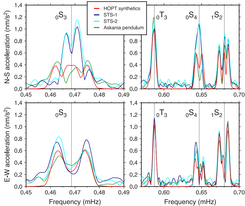
Figure B1. Spectra of data obtained from 120 hr time-series after the Aceh quake from the STS-1, STS-2 and Askania tiltmeter and of the corresponding synthetics (see Section 4). Time-series start at 2:30:00.0 hr UTC on 2004 December 26. Before computing the FFT, a Hann window was applied and the time-series padded with zeros. NS-components are shown in the top panels, EW-components at the bottom. The left panels show fundamental spheroidal mode {}_0S_3 , the panels on the right the group fundamental toroidal mode {}_0T_3 , fundamental spheroidal mode {}_0S_4 and spheroidal overtone {}_1S_2 .
