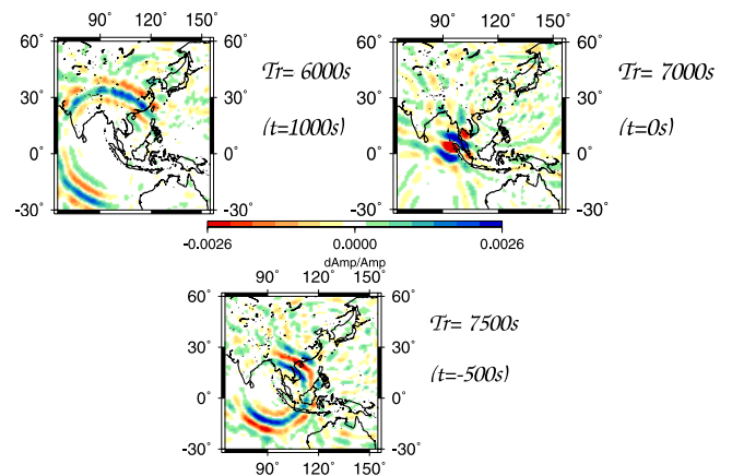
Figure 2. Vertical component of the time-reversed field at different times for the giant Sumatra-Andaman event. t is the absolute real time; T_r is the reversed time and T_r = 7000 s corresponds to source initial time ( t = 0 s).
