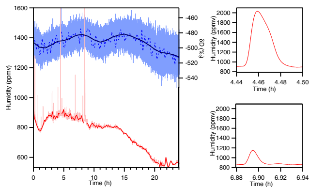
Figure 5. Left: example of raw data measured by the Picarro. Humidity (light red, ppmv) and \delta D (light blue, ‰), data averaged over 10 min for humidity (red, ppmv) and over 1 h for \delta D (dashed line blue, ‰) and over 1 h for \delta D (dark blue, ‰). Right: zoom on two “precipitation events” identified in the humidity signal of the Picarro (top, snow flake; bottom, diamond dust).
