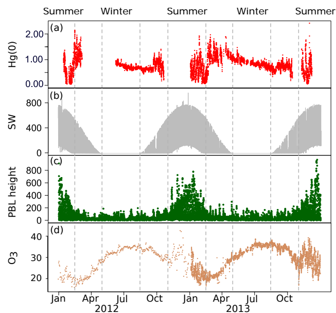
Figure 3. Annual variation in 2012 and 2013 of (a) hourly averaged Hg(0) concentrations (in \text{ng m}^{-3} ) at 500 and 25 cm above the snow surface in 2012 and 2013, respectively, (b) downwelling shortwave (SW) radiation (in \text{W m}^{-2} ), (c) planetary boundary layer (PBL) height (in m), and (d) ozone ( \text{O}_3 , daily mean in 2012 and hourly mean in 2013) mixing ratios (in ppbv). The vertical dashed lines represent seasonal boundaries.
