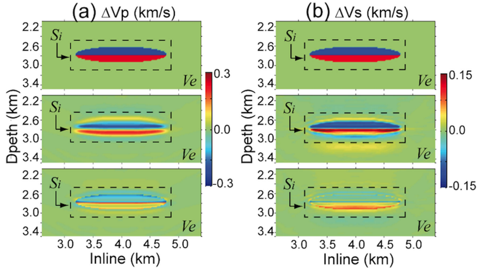
Figure 7. Vertical slices of inverted P -wave (a) and S -wave (b) velocity perturbations in the case of full domain FWI. The slices spread through the middle of the crossline direction shown in Fig. 6 and highlighted by the thick black boundary. The corresponding slices are the true (top), recovered (middle) and the residual (bottom) velocity perturbation.
