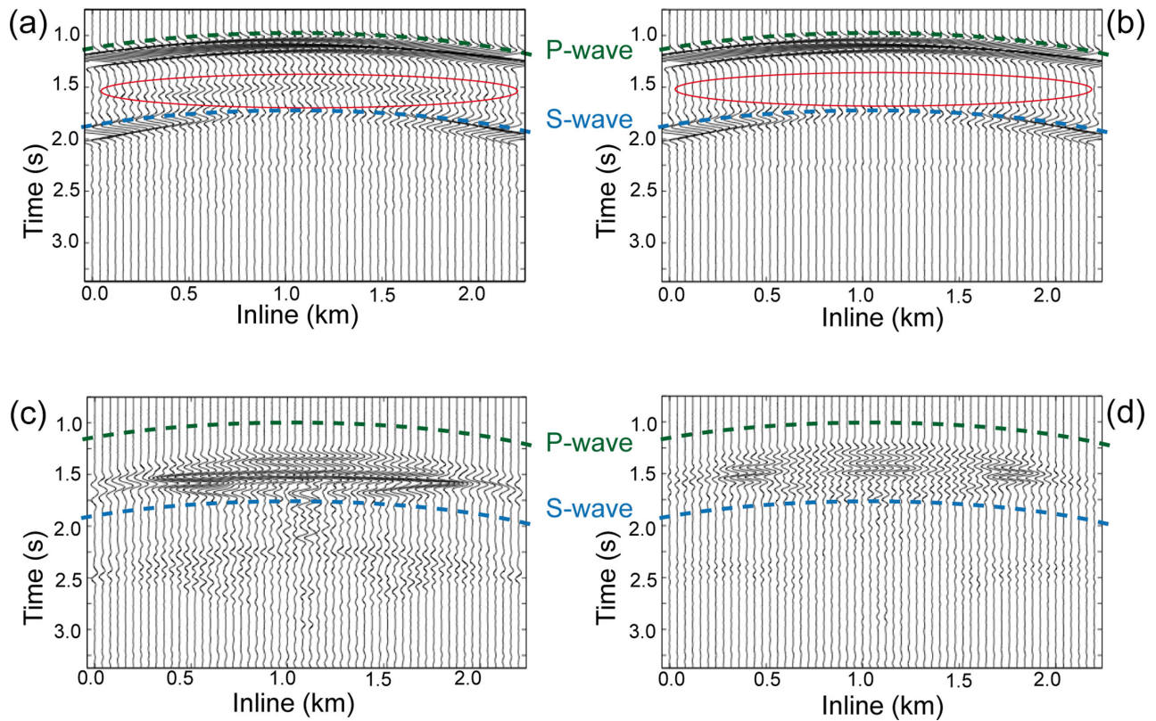
Figure 13. Vertical velocity component ( v_z ) recorded at receiver's position in localized FWI: (a) before perturbations; (b) after perturbations; (c) the difference between (a) & (b); (d) after final FWI residuals after 30 iterations; (c) & (d) are shown on the scale increased five times in comparison with (a) & (b).
