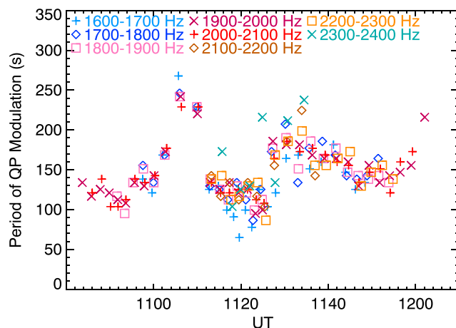
Figure 7. Modulation period (i.e., the time separation of two consecutive QP elements) observed by Kannuslehto as a function of time. Individual color symbols correspond to different frequency ranges, following the insert at the top.
