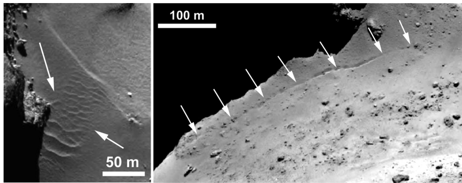
Figure 17. Examples of features detected on the neck. (a) Enlarged view showing a field of iso-oriented dune-like forms. (b) Enlarged view of an \sim 440 -m-long crack detected on the neck region (indicated by white arrows). This fracture seems to be constituted of aligned pits.
