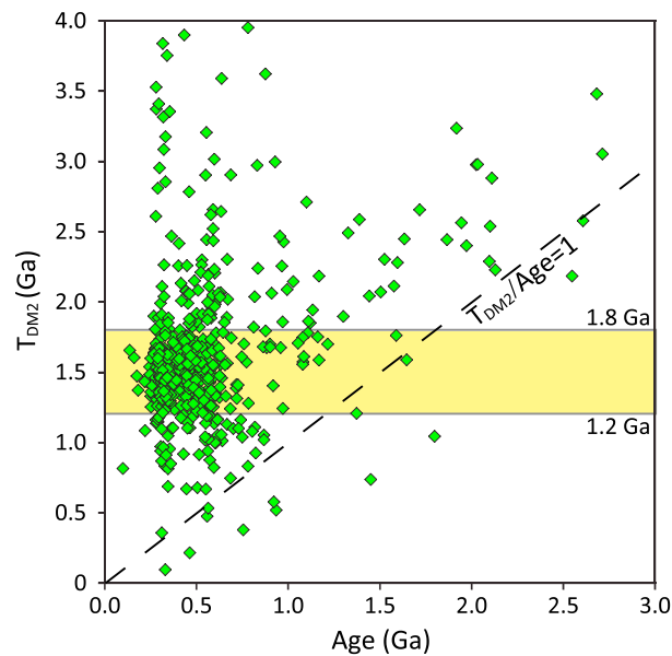
Figure 7. The two stage model Hf age T_{DM2} versus age plot for detrital zircons, showing the source of zircons. Most of the zircon Hf model ages are older than their crystallization ages, indicating a formation from remelting of older crustal rocks crystallized during previous events.
