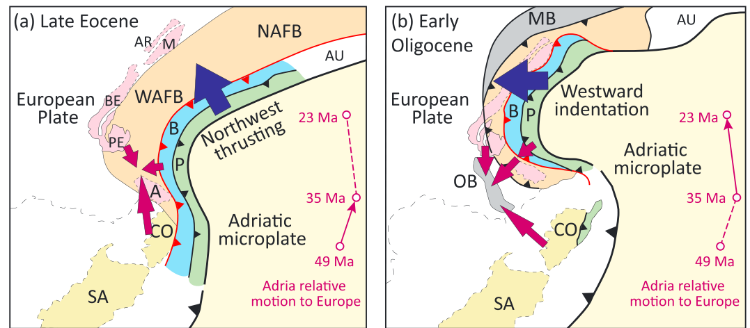
Figure 9. Late Eocene (a) and Early Oligocene (b) paleogeographic maps of the Western Alps showing the source areas for the terrigenous material, including the directions of sediment supply in the syntectonic sedimentary basins (modified after Dumont et al. [2011] and Malusà et al. [2015]). Adria motion relative to Europe is from Jolivet and Faccenna [2000]. A: Argentera. AR: Aiguilles Rouges. AU: Austroalpine Unit. B: Briançonnais Zone. BE: Belledonne. CO: Corsica. M: Mont Blanc. MB: Molasse Basin. NAFB: North Alpine Foreland Basin. OB: Oligocene Basins including the Digne, Devoluy and Barrême Basins. P: Piemonte Zone. PE: Pelvoux. SA: Sardinia. WAFB: Western Alpine Flexural Basin.
