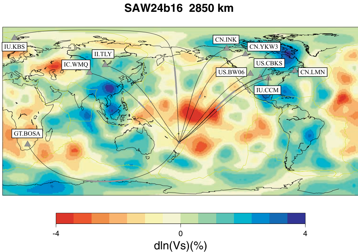
Figure 8. Configuration of source and stations used in this example. The background model is the tomographic model SAW24B16 above the CMB. The path between the source and stations are plotted, and in bold is plotted the part of the path that would sample the D'' layer in PREM.
