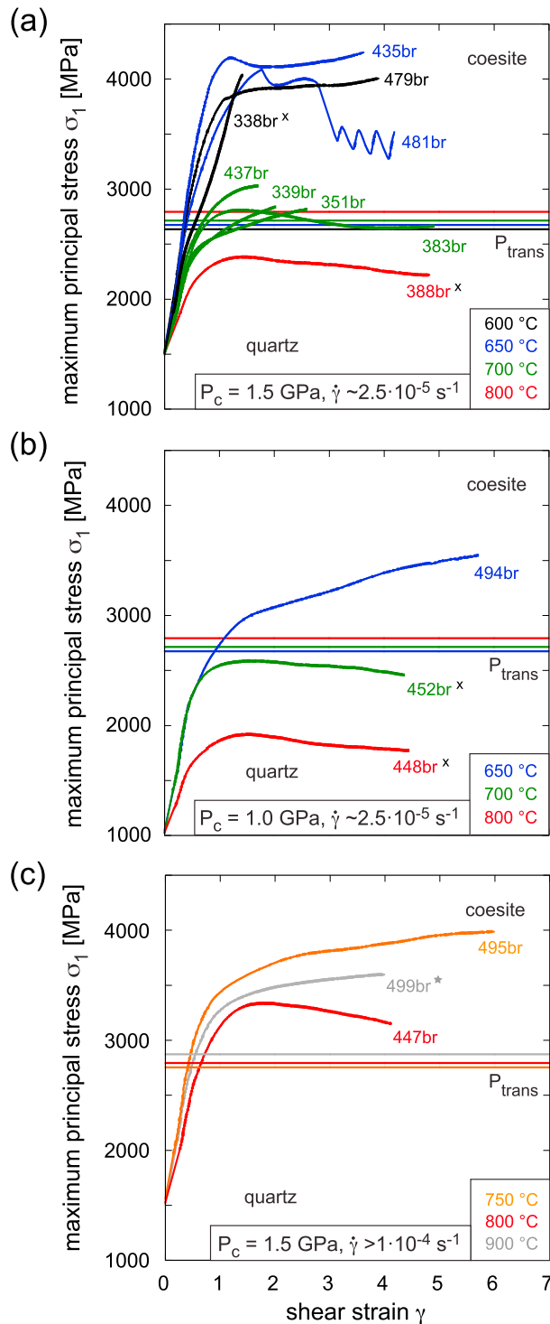
Figure 4. Maximum principal stress as a function of shear strain. The transformation pressure, P_{trans} , of the quartz-to-coesite phase transformation [after Bohlen and Boettcher, 1982 ] is marked by a horizontal line, color coded for each temperature. All samples, except those marked with a cross contain coesite. (a) Samples deformed at 1.5 GPa confining pressure and shear strain rates of \sim 2.5 \cdot 10^{-5} s^{-1} . (b) Samples deformed at 1.0 GPa confining pressure and shear strain rates of \sim 2.5 \cdot 10^{-5} s^{-1} . (c) Samples deformed at 1.5 GPa confining pressure and shear strain rates of \sim 1 \cdot 10^{-4} s^{-1} . The star at 499br indicates an even faster strain rate of \sim 1 \cdot 10^{-3} s^{-1} .
