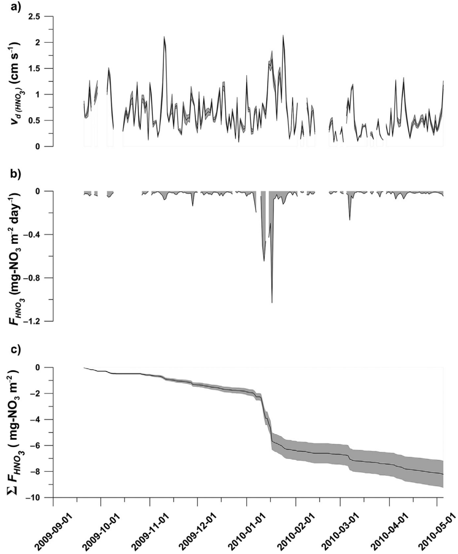
Fig. 5. Modelled dry deposition of \text{HNO}_3 during Winter 2009–2010: a) daily average deposition velocity ( v_d(\text{HNO}_3) ) given by the model, b) daily average dry deposition of \text{HNO}_3 ( F_{\text{HNO}_3} ) calculated from the C_{\text{HNO}_3} (Fig. 4a) and v_d(\text{HNO}_3) , and c) the accumulated dry deposition ( \Sigma F_{\text{HNO}_3} ) giving the total deposition for the winter season. The shaded areas in a) and c) indicate standard error of the estimates, while the shaded area in b) resembles the integrated area for the estimated dry deposition.
