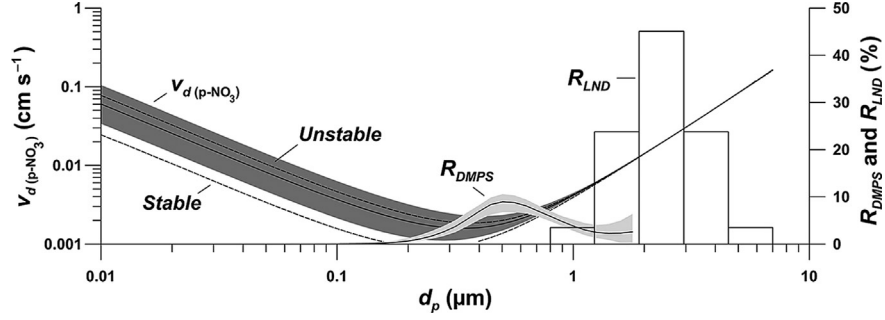
Fig. 7. Particulate median dry deposition velocities, v_d(p\text{-NO}_3) , for all particle diameters, d_p , estimated by the model and the corresponding median when only stable ( R_i > 0 ) or unstable ( R_i < 0 ) atmospheric conditions have been included (lower and upper dashed lines). The aerosol volume fraction, R_{\text{DMPS}} , measured by the Differential Mobility Particle Sizer (DMPS) at the Zeppelin atmospheric monitoring station, and the ratio, R_{\text{LND}} , between the five lognormal distributed (LND) size bins used to evaluate dry deposition of supermicron particles are also given. Shaded areas indicate 1st and 3rd quartiles of modelled output and measured R_{\text{DMPS}} .
