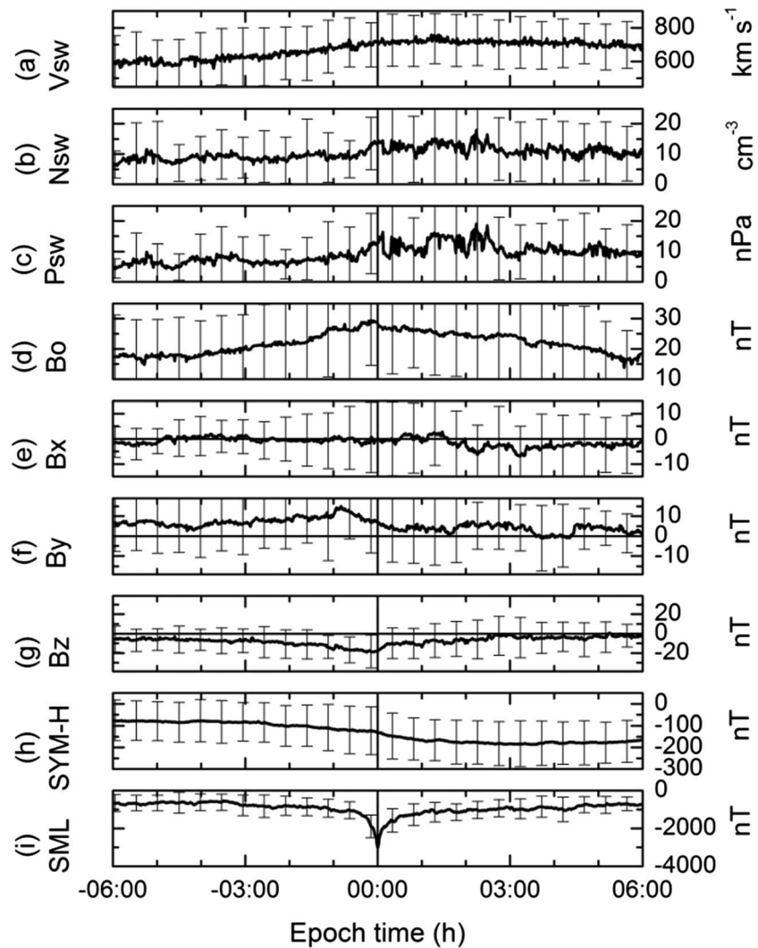
Figure 6. Superposed solar wind plasma variation during 24 isolated SSS events. From top to bottom, the panels show (a) V_{sw} ( \text{km s}^{-1} ), (b) N_{sw} ( \text{cm}^{-3} ), (c) P_{sw} (nPa), (d) IMF B_o (nT), (e) the B_x (nT), (f) B_y (nT) and (g) B_z (nT) components in GSM coordinates, and (h) the SYM-H (nT) and (i) SML (nT) indices. The zero epoch time corresponds to the peak SML strength of the SSS events. The curves show the average values (1 min time resolution), while the vertical bars show the standard deviations at 30 min intervals.
