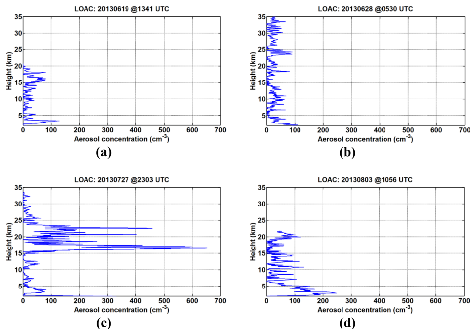
Figure 1. 50 m interpolated vertical profiles of aerosol concentration ( \text{cm}^{-3} ) with diameters 0.2–50 \mu\text{m} above Minorca Island (39.99° N, 4.25° E) (a–b) on 19 June at 13:41 UTC and 28 June at 05:30 UTC respectively, and above Ile du Levant (43.02° N, 6.46° E) (c–d) on 27 July at 23:03 UTC and 3 August at 10:56 UTC during the 2013 ChArMEX campaign.
