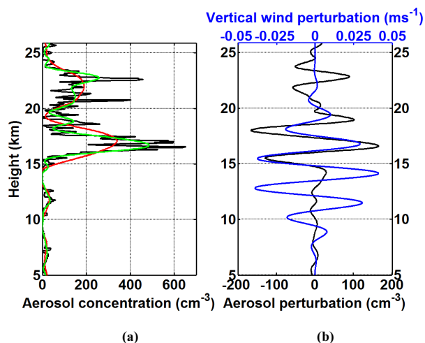
Figure 11. Vertical profiles of (a) aerosol concentration ( \text{cm}^{-3} ) and (b) aerosol (size class: 0.2\text{--}50\ \mu\text{m} ) perturbations with 1.6\text{--}3.2\ \text{km} vertical wavelengths and simulated vertical wind perturbations ( \text{ms}^{-1} ) on 27 July at 23:03 UTC. On left panel, black (red) solid line corresponds to raw (background) profile ( \text{cm}^{-3} ). The sum of the background profile and GW-induced perturbations is drawn as a green solid line.
