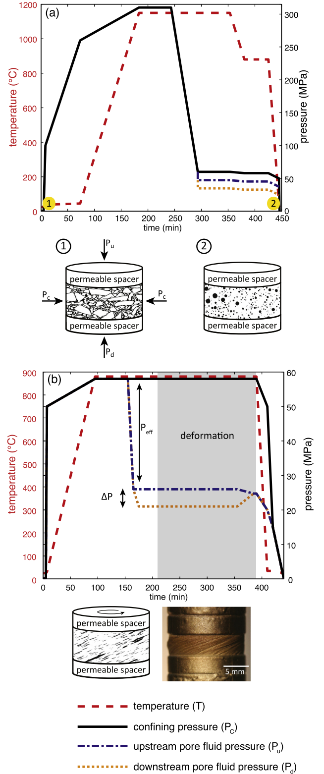
Fig. 3. Schematic representation of the experimental conditions for (a) starting material synthesis and (b) deformation of the bubble-bearing magmas in simple shear (see text for details). (a) Sample schematics show the powdered sample before synthesis (1) and after synthesis (2). (b) The grey box indicates when deformation occurred, after the sample was brought to equilibrium with the pressure and temperature conditions. In this example, the pore fluid pressures equilibrate across the sample, representing permeability development. Deformation is in right lateral shear. The sample picture is of experiment PP512, after deformation.
