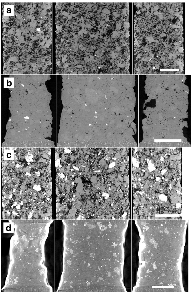
Fig. 3. Vertical slice images of (a), (c) starting columnar samples and (b), (d) run products after the heating experiment (PP400 and PP486) obtained by X-ray CT. (a), (b) and (c), (d) images represent the MY and MO samples, respectively. The centre images represent the longitudinal axis images of columnar samples, and the right and left images correspond to longitudinal tangential sections (Paterson and Olgaard, 2000). In (d), an iron jacket (white area on the sample) surrounds the run product, and porous alumina spacers are found at the top and bottom. The fraction of pores (black portions in the sample) was high before heating experiments, although it strongly decreased after heating and deformation. The white scale bar is 5 mm long.
