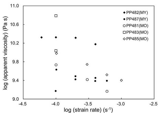
Fig. 7. Dependence of apparent viscosity on strain rate. The low crystallinity sample (MY) shows no clear dependence on the strain rate, whereas the viscosity decreases with the strain rate at high crystallinity (MO). Even with the same sample, the viscosity shows large variation when a crystal network is locally formed.
