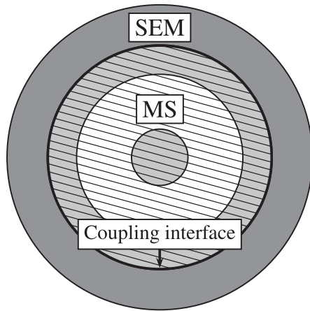
Figure 1. The Earth model is partitioned in two parts: the SEM is used in the outer shell, the Modal Solution is used in the inner sphere and is coupled with the SEM on a spherical interface.
