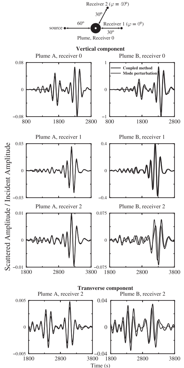
Figure 5. Comparison between the scattered field computed by the coupled method (solid line) and the perturbation method (dotted line), for plume A (left) and plume B (right), at receivers 0, 1 and 2. The receiver positions are shown on the top sketch.
