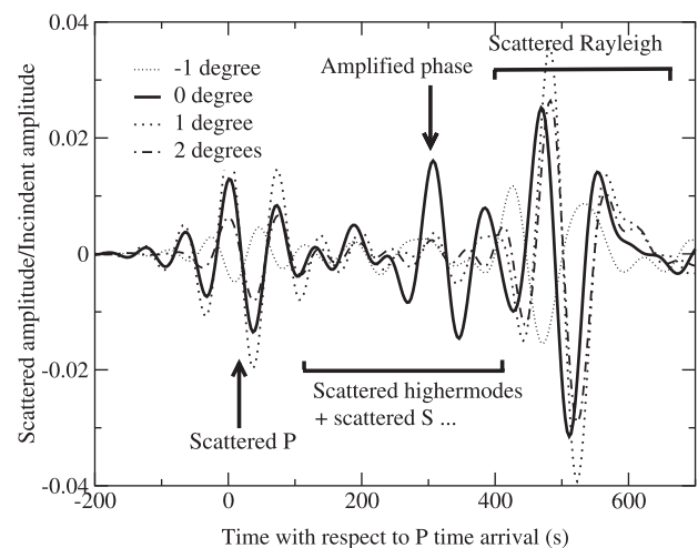
Figure 4. Vertical component of the scattered field for the small plume (plume 1), at four angular distances along the source-plume great circle: -1 , 0 , 1 and 2 degrees from the plume. The arrow indicates a scattered amplified phase for the receiver on top of the plume.
