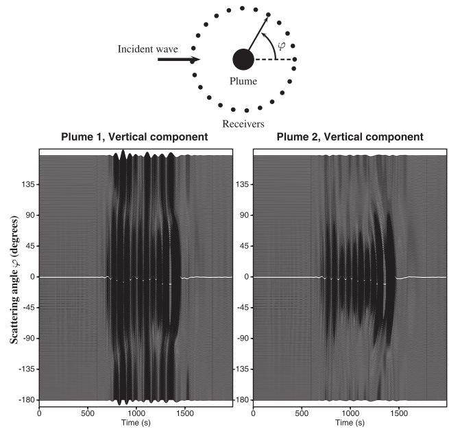
Figure 3. Vertical component of the scattered field, as a function of the scattering angle \varphi , as detailed by the top sketch, for two plume-like cylindrical structures of 100 km radius (left) and 250 km radius (right). The forward scattering pattern increases with the plume radius. The maximum scattering amplitude is related to surface waves.
