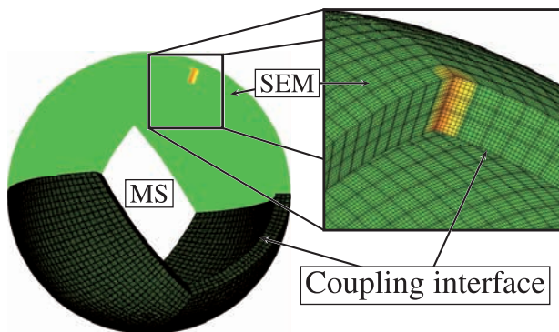
Figure 2. Left: global view of the model where two regions have been removed for sake of visibility. The SEM mesh is drawn only for two regions. Right: zoom on the plume inclusion area. The colors indicate the S wave velocity contrast with respect to the modified PREM model. On this figure, the plume radius is of 250 km and the maximum S-velocity contrast is 4.5%.
