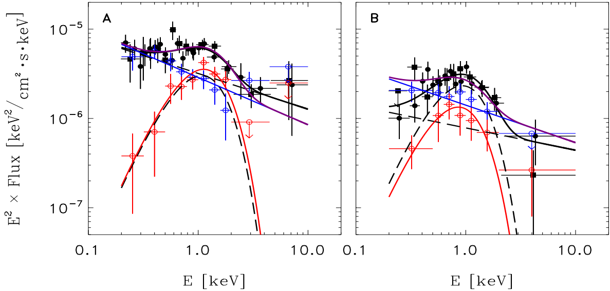
FIG. 4.— Results of the ML spectroscopy for the Q-mode (left panel) and B-mode (right panel). Black lines and points refer to the 2D-ML (circles pn, squares sum of the two MOS), solid lines are the best-fit blackbody plus power law models, dashed lines the individual components). The results of the 3D-ML analysis are in blue for the unpulsed component (data points and best-fit with a single power-law) and in red for the pulsed component (data points and best-fit with a single blackbody). The purple line is the sum of the blue and red lines.
