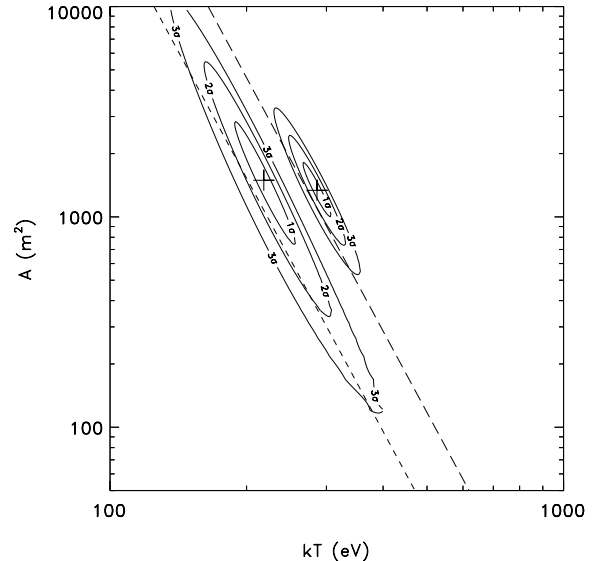
FIG. 7.— Confidence regions ( 1\sigma , 2\sigma , and 3\sigma c.l.) of blackbody temperature and emitting area for the pulsed thermal component of the B-mode (bottom-left contours) and Q-mode (top-right contours). The dashed lines correspond to bolometric luminosities of 10^{29} and 3 \times 10^{29} erg s^{-1} , for a distance of 630 pc.
